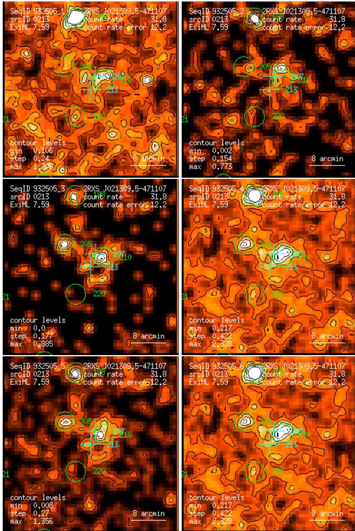
Figure 213: RASS 932505: detection 0213: band rate images, Gaussian filter: (1) PSPC channels 11 – 41, (2) 52 – 90, (3) 91 – 201, (4) 11 – 235, (5) 52 – 201, (6) 11 – 201. Broad band rates in counts/ks. Band rate contour levels in counts/ks/arcmin 2 .
