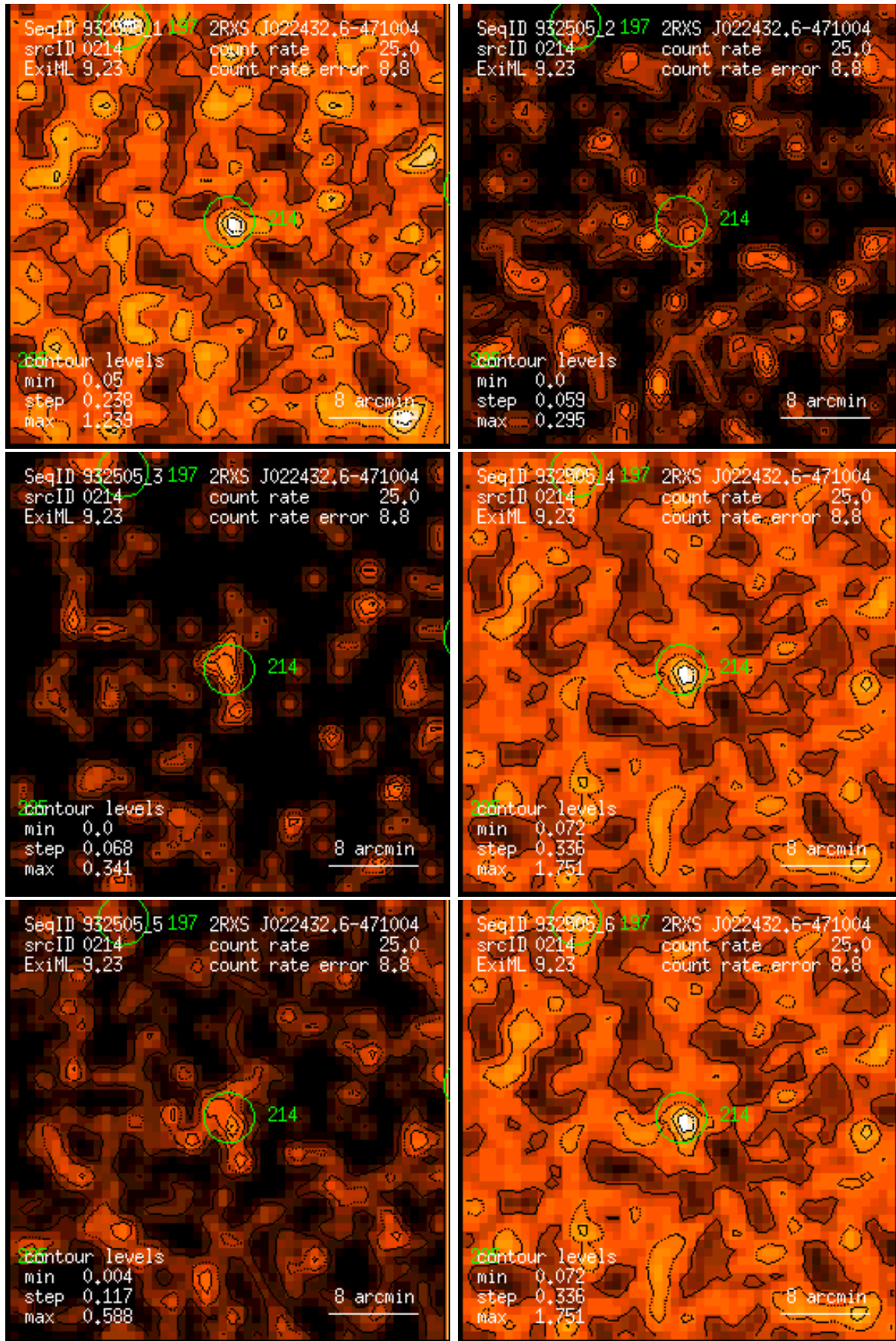
Figure 214: RASS 932505: detection 0214: band rate images, Gaussian filter: (1) PSPC channels 11 – 41, (2) 52 – 90, (3) 91 – 201, (4) 11 – 235, (5) 52 – 201, (6) 11 – 201. Broad band rates in counts/ks. Band rate contour levels in counts/ks/arcmin 2 .
