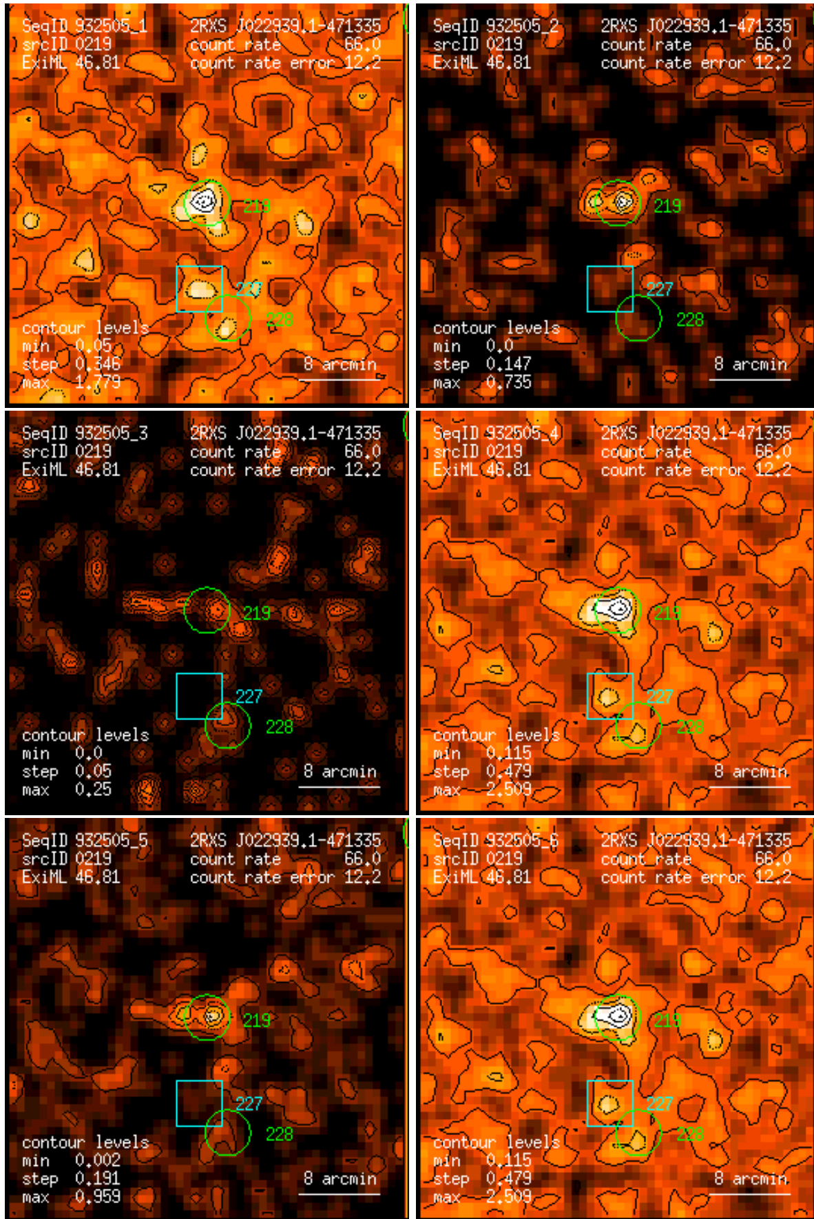
Figure 219: RASS 932505: detection 0219: band rate images, Gaussian filter: (1) PSPC channels 11 – 41, (2) 52 – 90, (3) 91 – 201, (4) 11 – 235, (5) 52 – 201, (6) 11 – 201. Broad band rates in counts/ks. Band rate contour levels in counts/ks/arcmin 2 .
