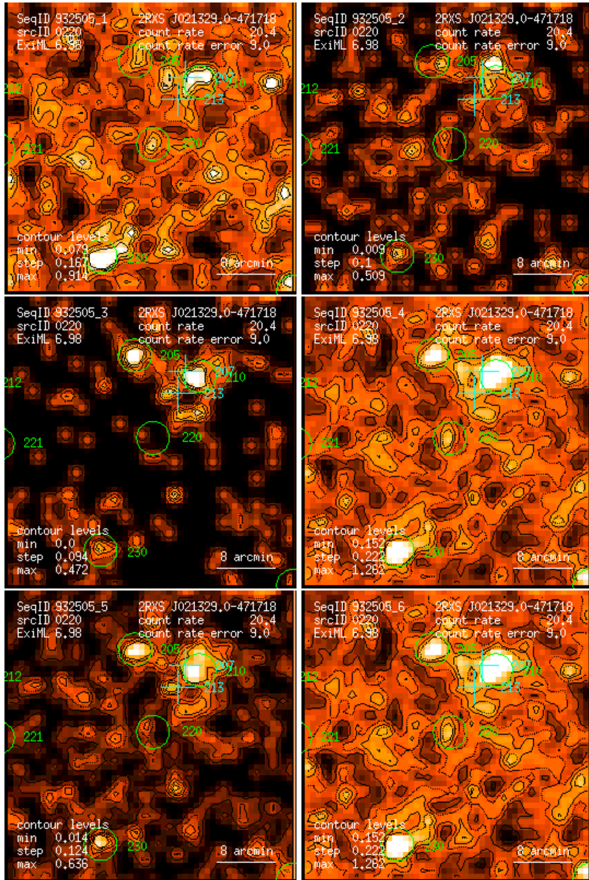
Figure 220: RASS 932505: detection 0220: band rate images, Gaussian filter: (1) PSPC channels 11 – 41, (2) 52 – 90, (3) 91 – 201, (4) 11 – 235, (5) 52 – 201, (6) 11 – 201. Broad band rates in counts/ks. Band rate contour levels in counts/ks/arcmin 2 .
