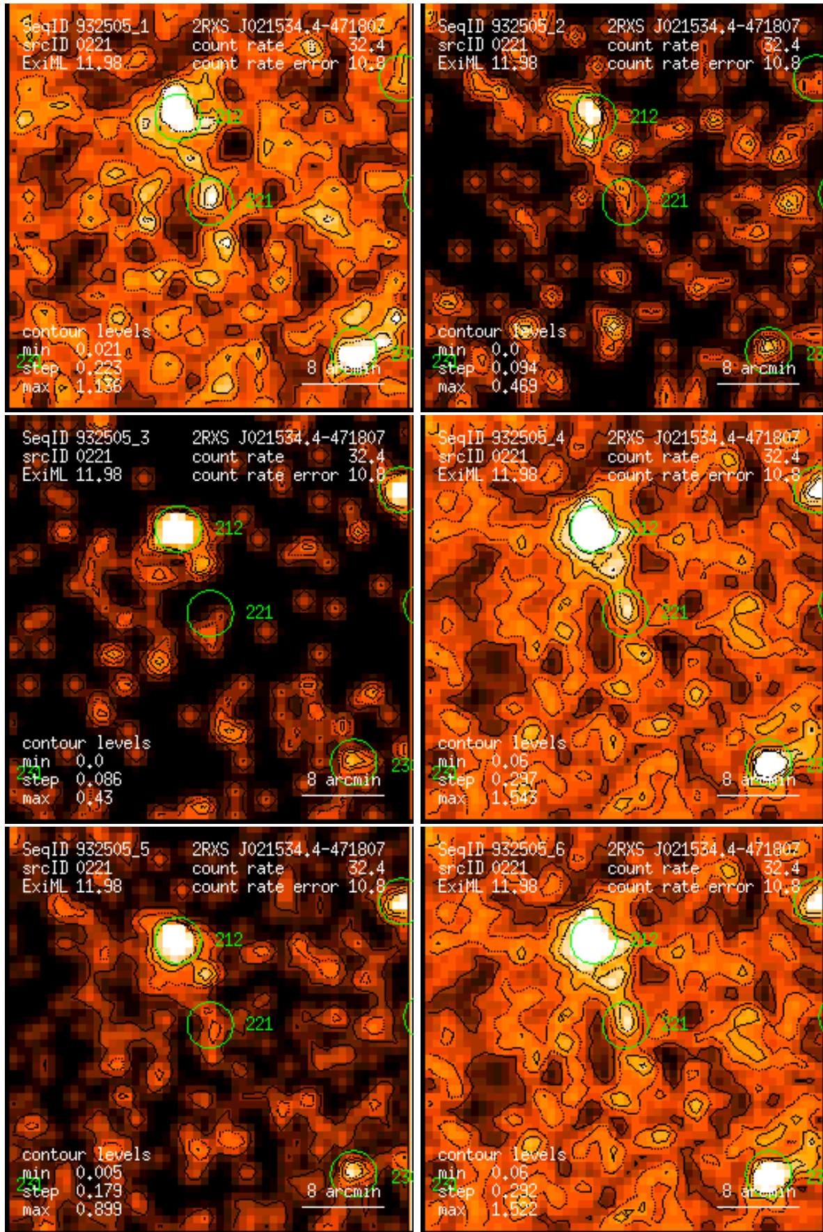
Figure 221: RASS 932505: detection 0221: band rate images, Gaussian filter: (1) PSPC channels 11 – 41, (2) 52 – 90, (3) 91 – 201, (4) 11 – 235, (5) 52 – 201, (6) 11 – 201. Broad band rates in counts/ks. Band rate contour levels in counts/ks/arcmin 2 .
