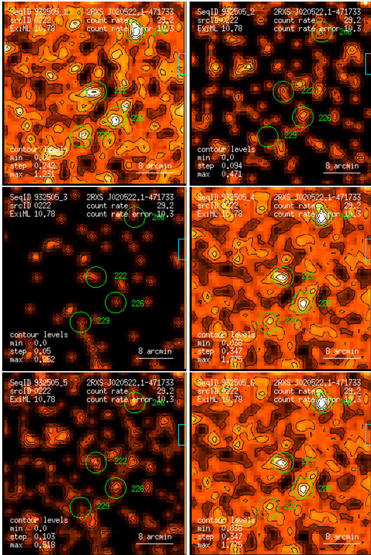
Figure 222: RASS 932505: detection 0222: band rate images, Gaussian filter: (1) PSPC channels 11 – 41, (2) 52 – 90, (3) 91 – 201, (4) 11 – 235, (5) 52 – 201, (6) 11 – 201. Broad band rates in counts/ks. Band rate contour levels in counts/ks/arcmin 2 .
