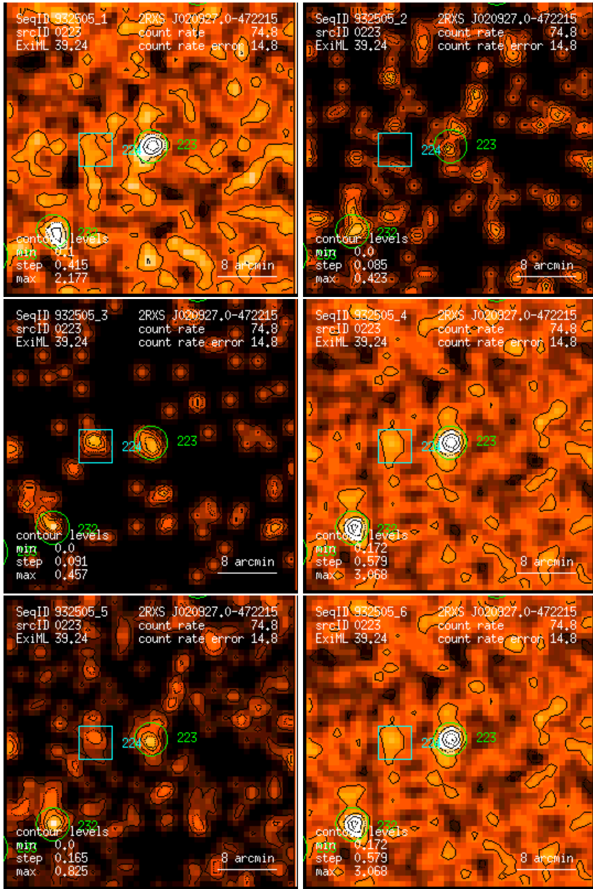
Figure 223: RASS 932505: detection 0223: band rate images, Gaussian filter: (1) PSPC channels 11 – 41, (2) 52 – 90, (3) 91 – 201, (4) 11 – 235, (5) 52 – 201, (6) 11 – 201. Broad band rates in counts/ks. Band rate contour levels in counts/ks/arcmin 2 .
