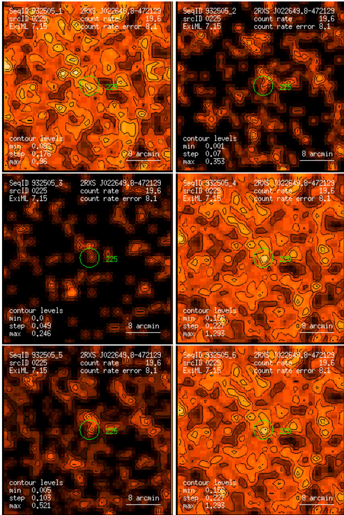
Figure 225: RASS 932505: detection 0225: band rate images, Gaussian filter: (1) PSPC channels 11 – 41, (2) 52 – 90, (3) 91 – 201, (4) 11 – 235, (5) 52 – 201, (6) 11 – 201. Broad band rates in counts/ks. Band rate contour levels in counts/ks/arcmin 2 .
