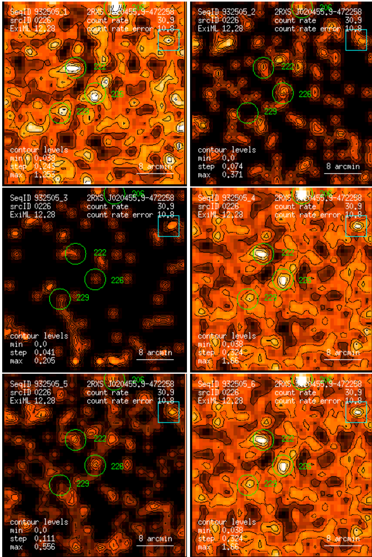
Figure 226: RASS 932505: detection 0226: band rate images, Gaussian filter: (1) PSPC channels 11 – 41, (2) 52 – 90, (3) 91 – 201, (4) 11 – 235, (5) 52 – 201, (6) 11 – 201. Broad band rates in counts/ks. Band rate contour levels in counts/ks/arcmin 2 .
