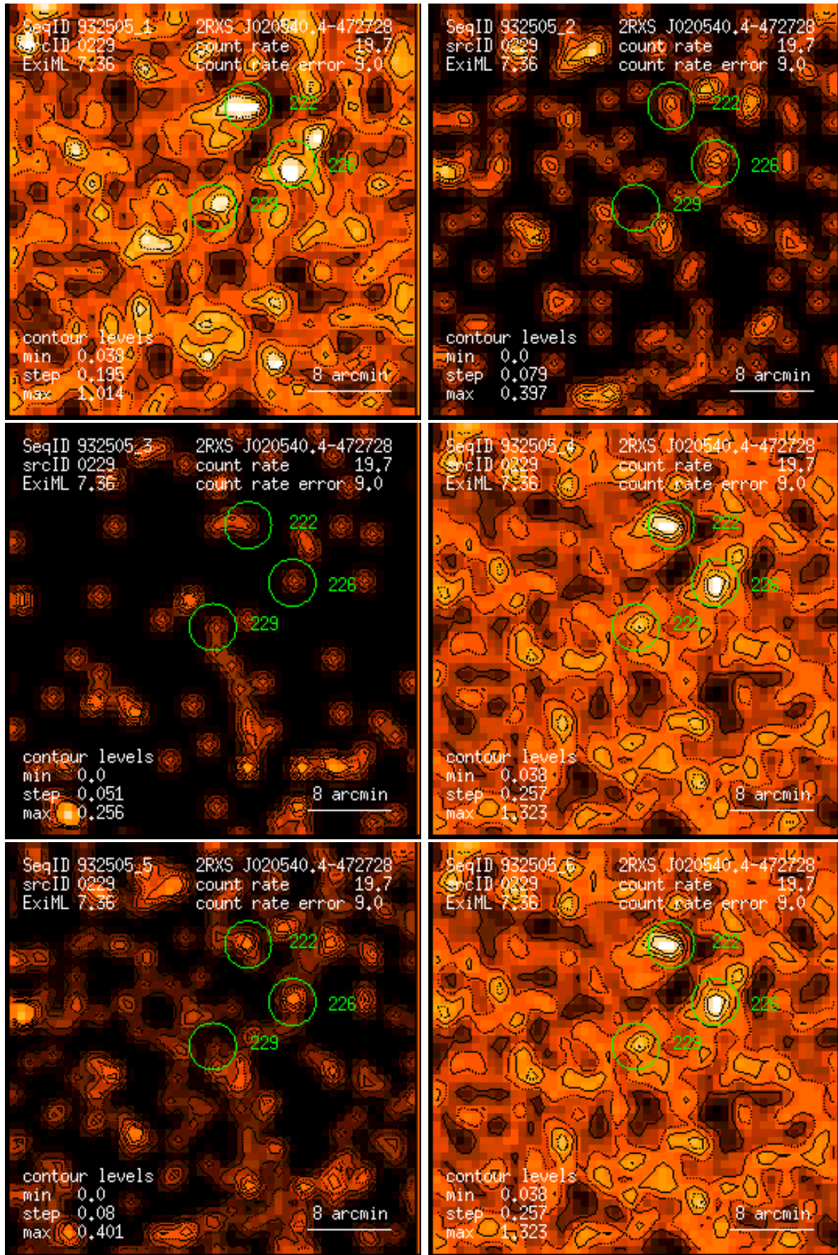
Figure 229: RASS 932505: detection 0229: band rate images, Gaussian filter: (1) PSPC channels 11 – 41, (2) 52 – 90, (3) 91 – 201, (4) 11 – 235, (5) 52 – 201, (6) 11 – 201. Broad band rates in counts/ks. Band rate contour levels in counts/ks/arcmin 2 .
