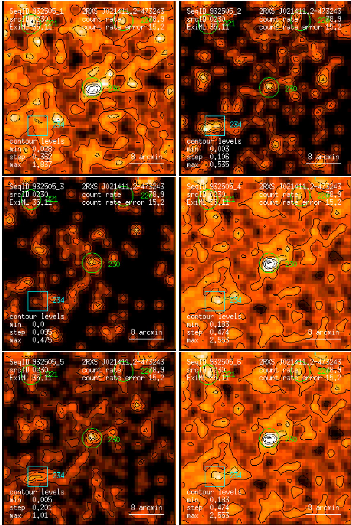
Figure 230: RASS 932505: detection 0230: band rate images, Gaussian filter: (1) PSPC channels 11 – 41, (2) 52 – 90, (3) 91 – 201, (4) 11 – 235, (5) 52 – 201, (6) 11 – 201. Broad band rates in counts/ks. Band rate contour levels in counts/ks/arcmin 2 .
