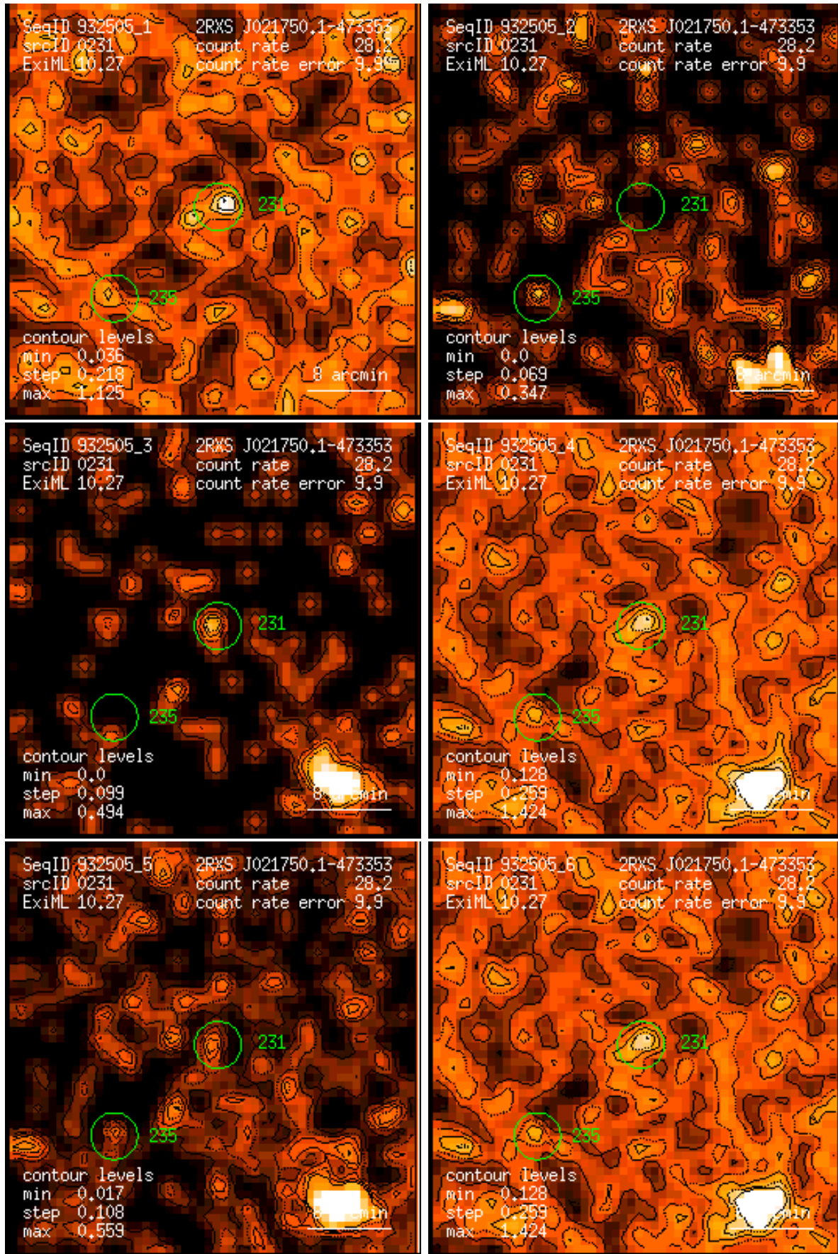
Figure 231: RASS 932505: detection 0231: band rate images, Gaussian filter: (1) PSPC channels 11 – 41, (2) 52 – 90, (3) 91 – 201, (4) 11 – 235, (5) 52 – 201, (6) 11 – 201. Broad band rates in counts/ks. Band rate contour levels in counts/ks/arcmin 2 .
