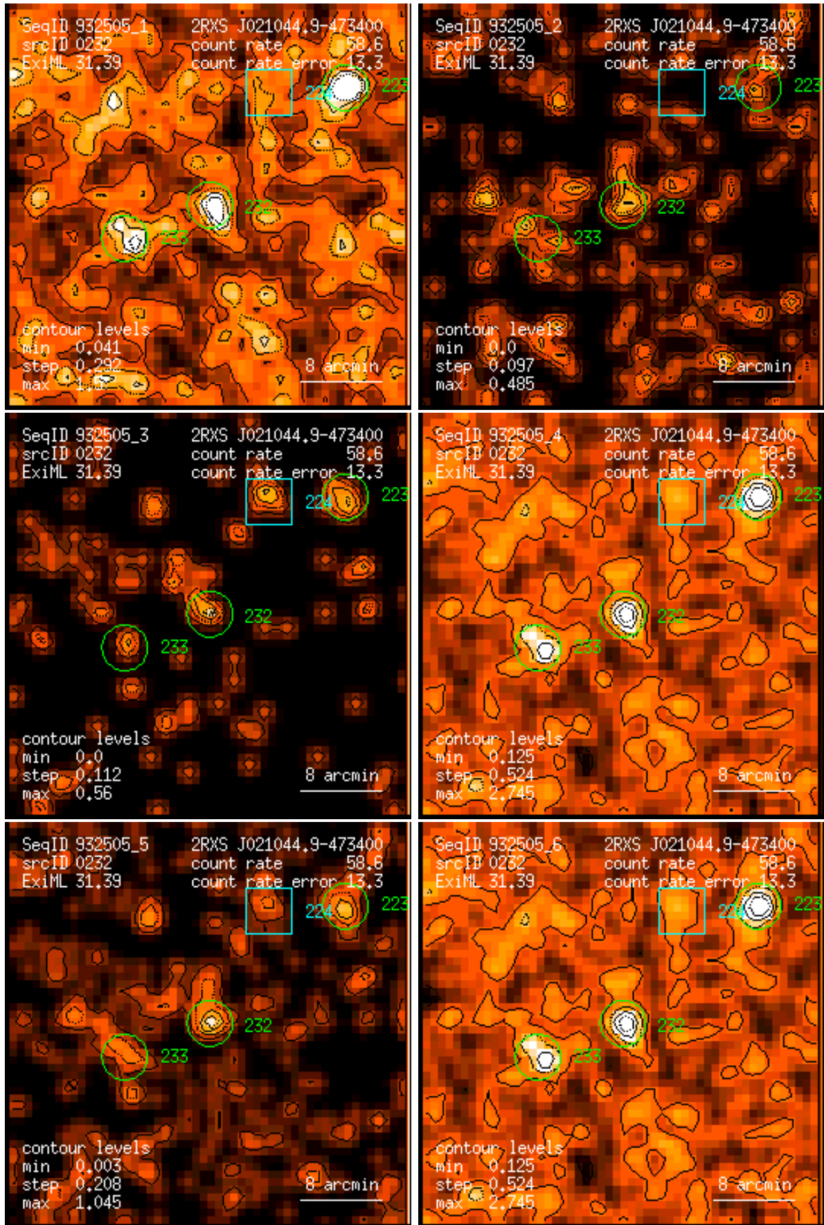
Figure 232: RASS 932505: detection 0232: band rate images, Gaussian filter: (1) PSPC channels 11 – 41, (2) 52 – 90, (3) 91 – 201, (4) 11 – 235, (5) 52 – 201, (6) 11 – 201. Broad band rates in counts/ks. Band rate contour levels in counts/ks/arcmin 2 .
