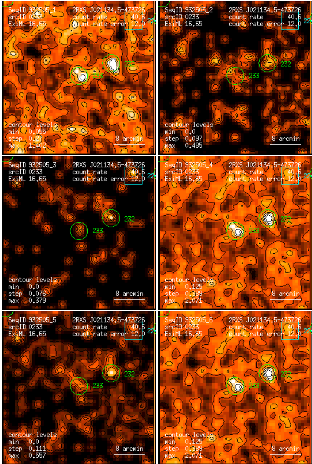
Figure 233: RASS 932505: detection 0233: band rate images, Gaussian filter: (1) PSPC channels 11 – 41, (2) 52 – 90, (3) 91 – 201, (4) 11 – 235, (5) 52 – 201, (6) 11 – 201. Broad band rates in counts/ks. Band rate contour levels in counts/ks/arcmin 2 .
