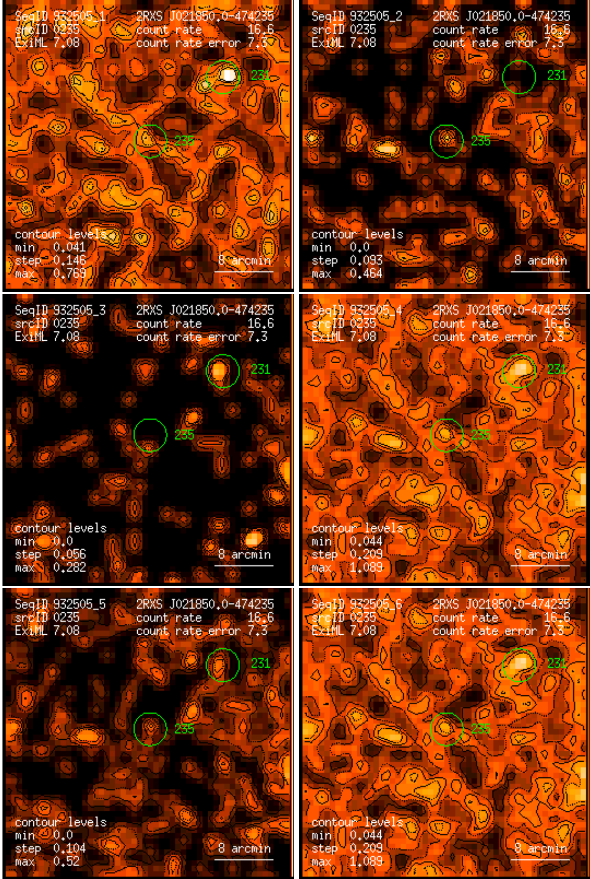
Figure 235: RASS 932505: detection 0235: band rate images, Gaussian filter: (1) PSPC channels 11 – 41, (2) 52 – 90, (3) 91 – 201, (4) 11 – 235, (5) 52 – 201, (6) 11 – 201. Broad band rates in counts/ks. Band rate contour levels in counts/ks/arcmin 2 .
