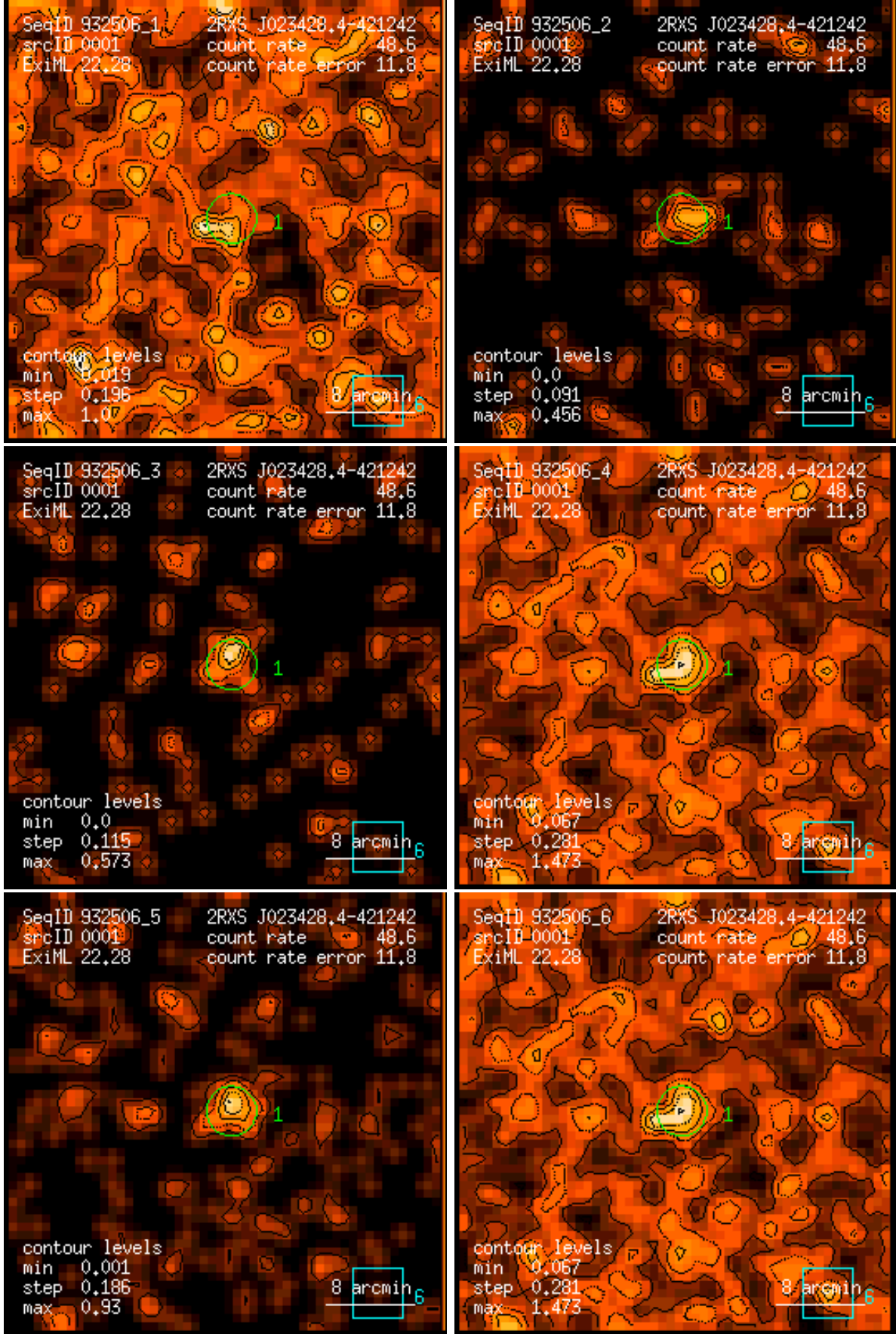
Figure 1: RASS 932506: detection 0001: band rate images, Gaussian filter: (1) PSPC channels 11 – 41, (2) 52 – 90, (3) 91 – 201, (4) 11 – 235, (5) 52 – 201, (6) 11 – 201. Broad band rates in counts/ks. Band rate contour levels in counts/ks/arcmin 2 .
