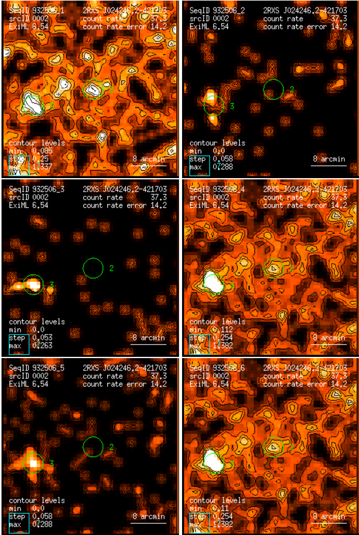
Figure 2: RASS 932506: detection 0002: band rate images, Gaussian filter: (1) PSPC channels 11 – 41, (2) 52 – 90, (3) 91 – 201, (4) 11 – 235, (5) 52 – 201, (6) 11 – 201. Broad band rates in counts/ks. Band rate contour levels in counts/ks/arcmin 2 .
