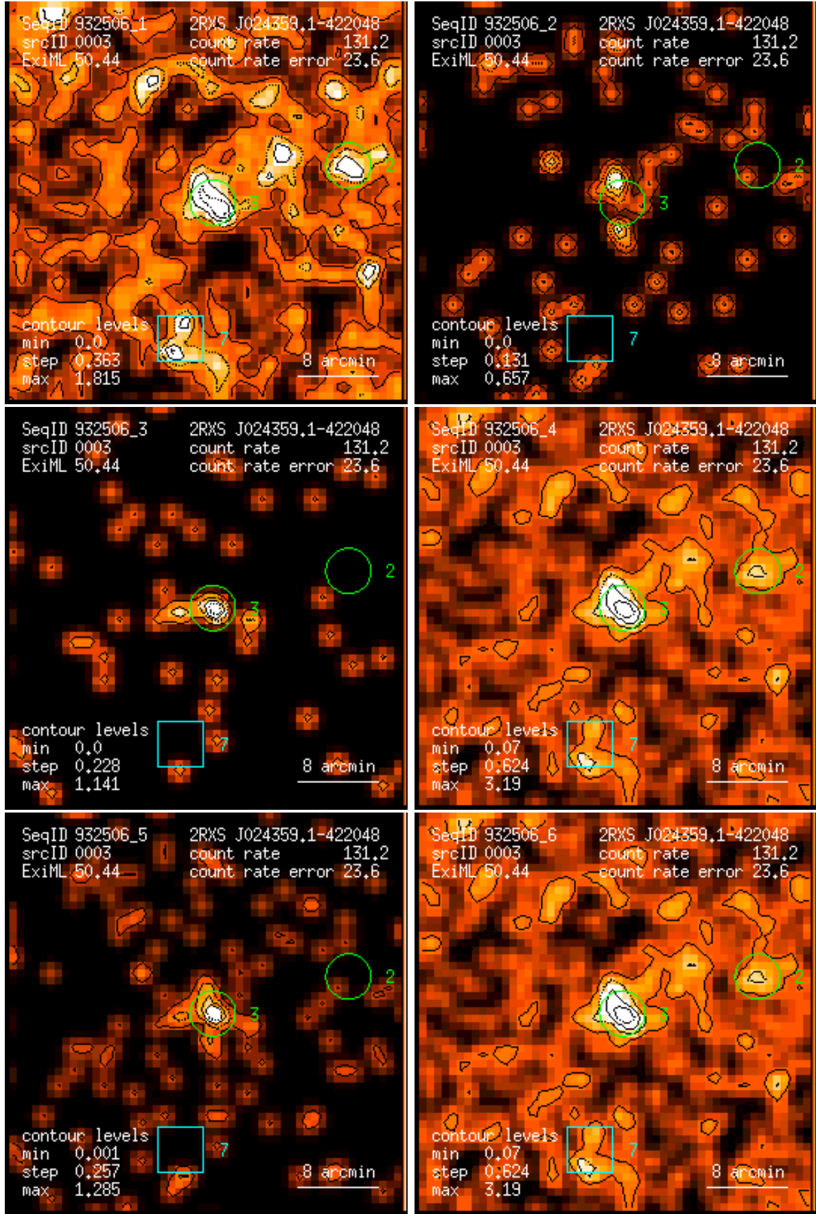
Figure 3: RASS 932506: detection 0003: band rate images, Gaussian filter: (1) PSPC channels 11 – 41, (2) 52 – 90, (3) 91 – 201, (4) 11 – 235, (5) 52 – 201, (6) 11 – 201. Broad band rates in counts/ks. Band rate contour levels in counts/ks/arcmin 2 .
