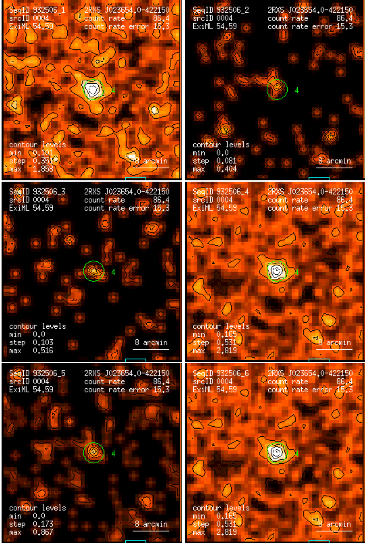
Figure 4: RASS 932506: detection 0004: band rate images, Gaussian filter: (1) PSPC channels 11 – 41, (2) 52 – 90, (3) 91 – 201, (4) 11 – 235, (5) 52 – 201, (6) 11 – 201. Broad band rates in counts/ks. Band rate contour levels in counts/ks/arcmin 2 .
