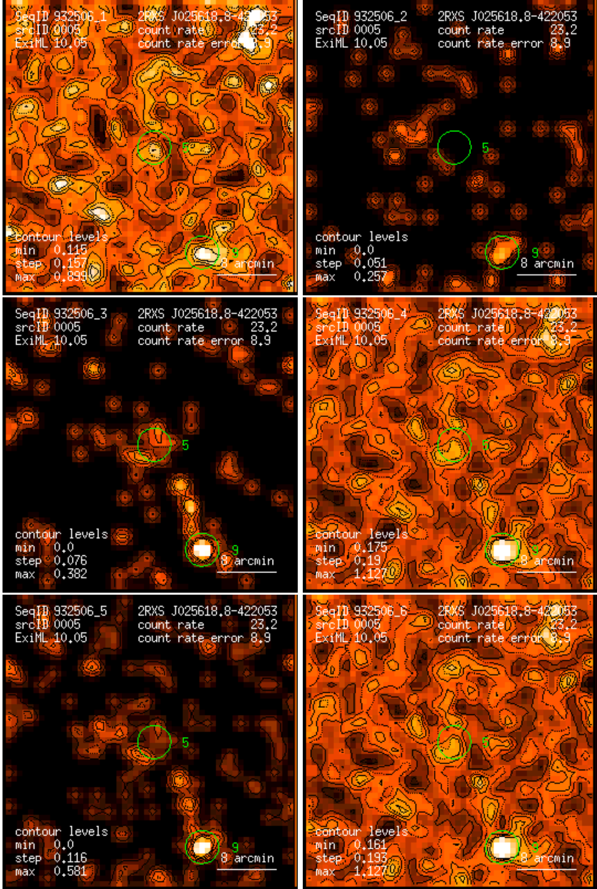
Figure 5: RASS 932506: detection 0005: band rate images, Gaussian filter: (1) PSPC channels 11 – 41, (2) 52 – 90, (3) 91 – 201, (4) 11 – 235, (5) 52 – 201, (6) 11 – 201. Broad band rates in counts/ks. Band rate contour levels in counts/ks/arcmin 2 .
