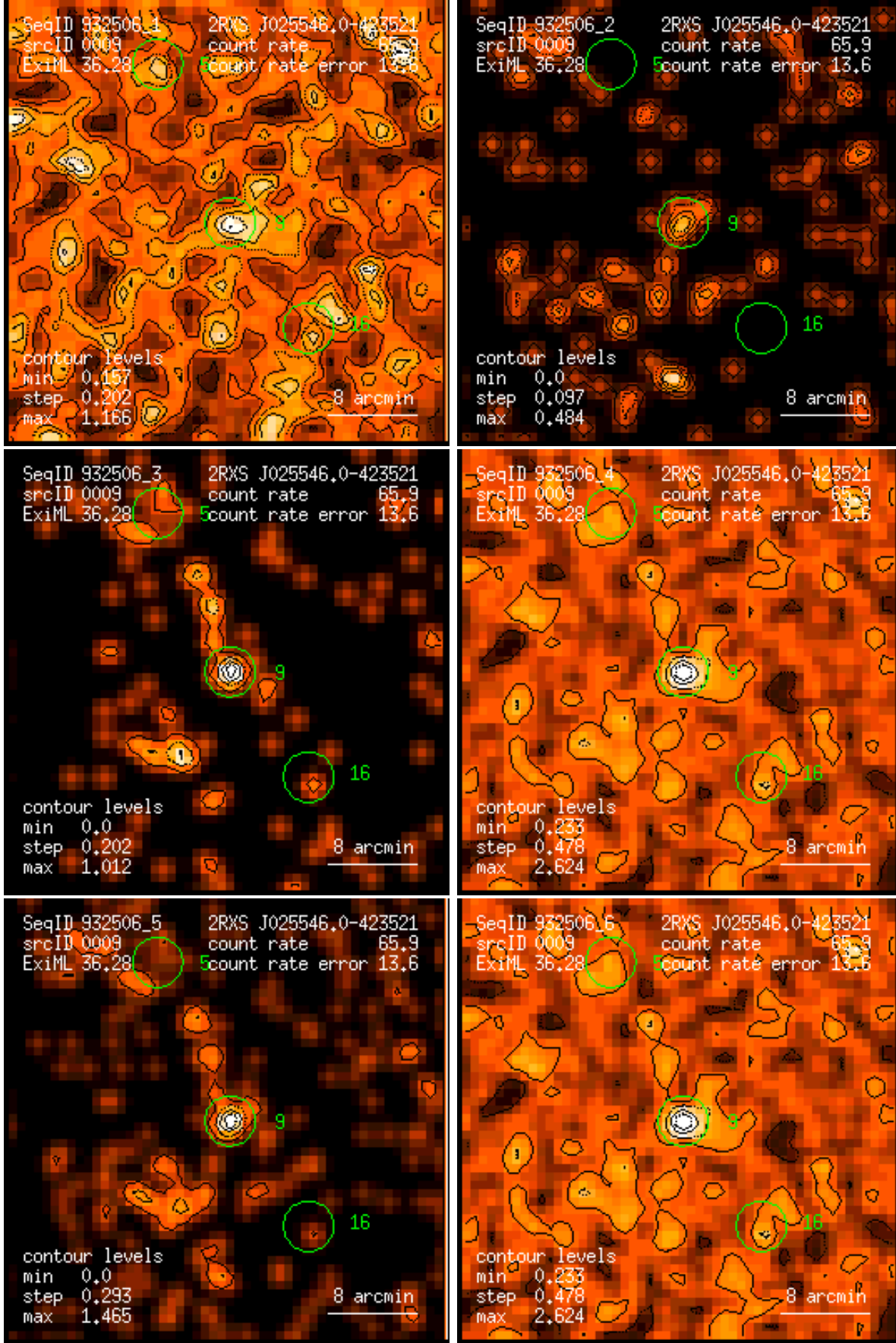
Figure 9: RASS 932506: detection 0009: band rate images, Gaussian filter: (1) PSPC channels 11 – 41, (2) 52 – 90, (3) 91 – 201, (4) 11 – 235, (5) 52 – 201, (6) 11 – 201. Broad band rates in counts/ks. Band rate contour levels in counts/ks/arcmin 2 .
