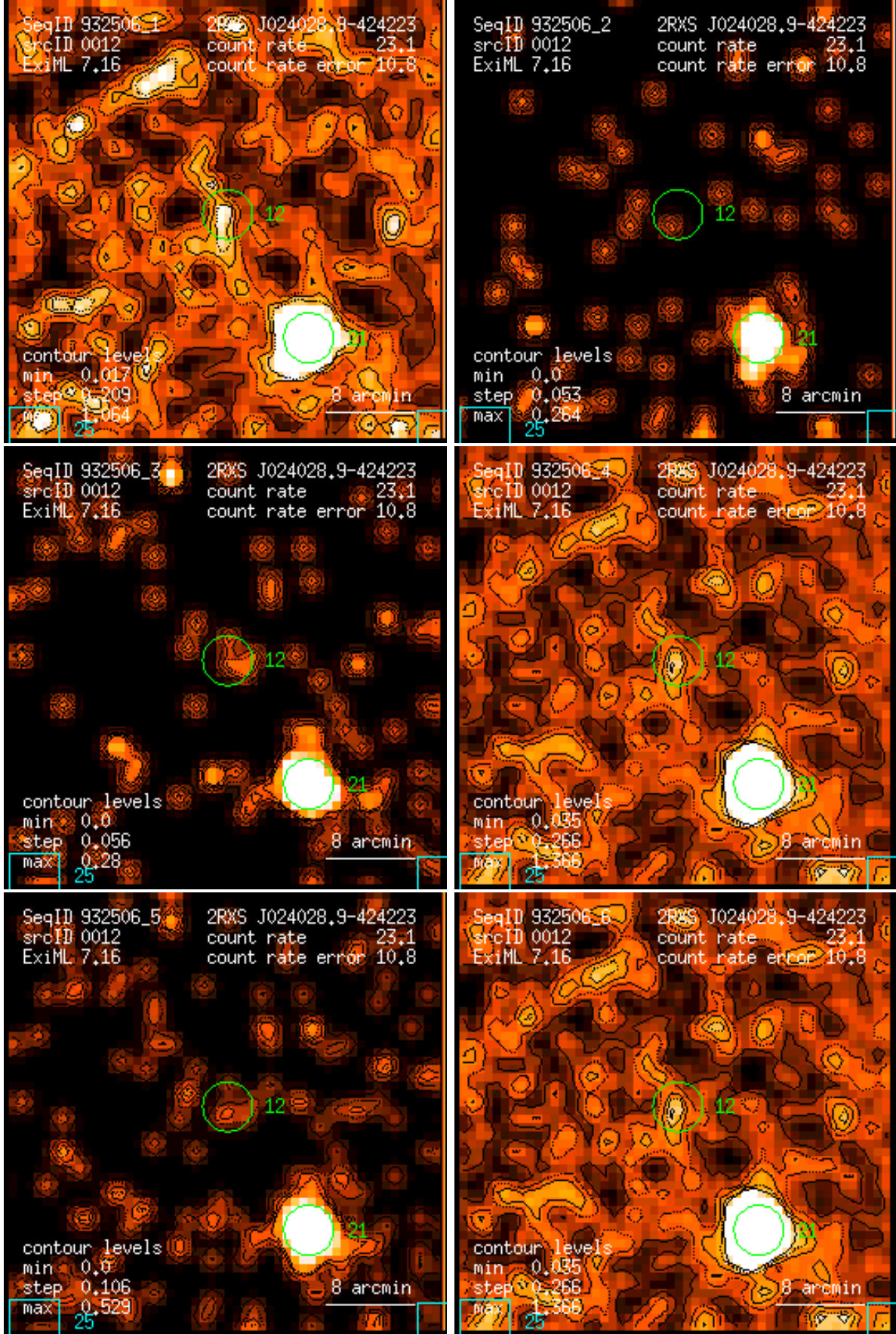
Figure 12: RASS 932506: detection 0012: band rate images, Gaussian filter: (1) PSPC channels 11 – 41, (2) 52 – 90, (3) 91 – 201, (4) 11 – 235, (5) 52 – 201, (6) 11 – 201. Broad band rates in counts/ks. Band rate contour levels in counts/ks/arcmin 2 .
