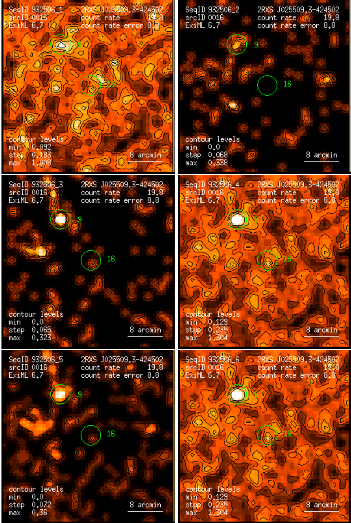
Figure 16: RASS 932506: detection 0016: band rate images, Gaussian filter: (1) PSPC channels 11 – 41, (2) 52 – 90, (3) 91 – 201, (4) 11 – 235, (5) 52 – 201, (6) 11 – 201. Broad band rates in counts/ks. Band rate contour levels in counts/ks/arcmin 2 .
