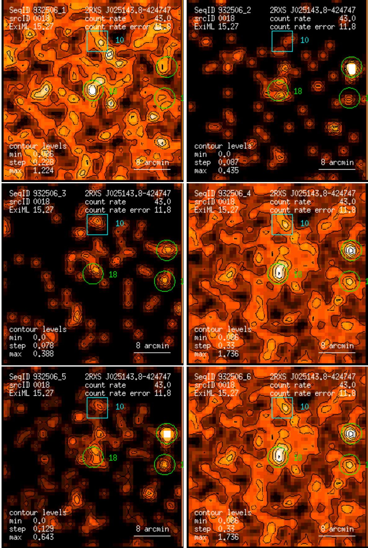
Figure 18: RASS 932506: detection 0018: band rate images, Gaussian filter: (1) PSPC channels 11 – 41, (2) 52 – 90, (3) 91 – 201, (4) 11 – 235, (5) 52 – 201, (6) 11 – 201. Broad band rates in counts/ks. Band rate contour levels in counts/ks/arcmin 2 .
