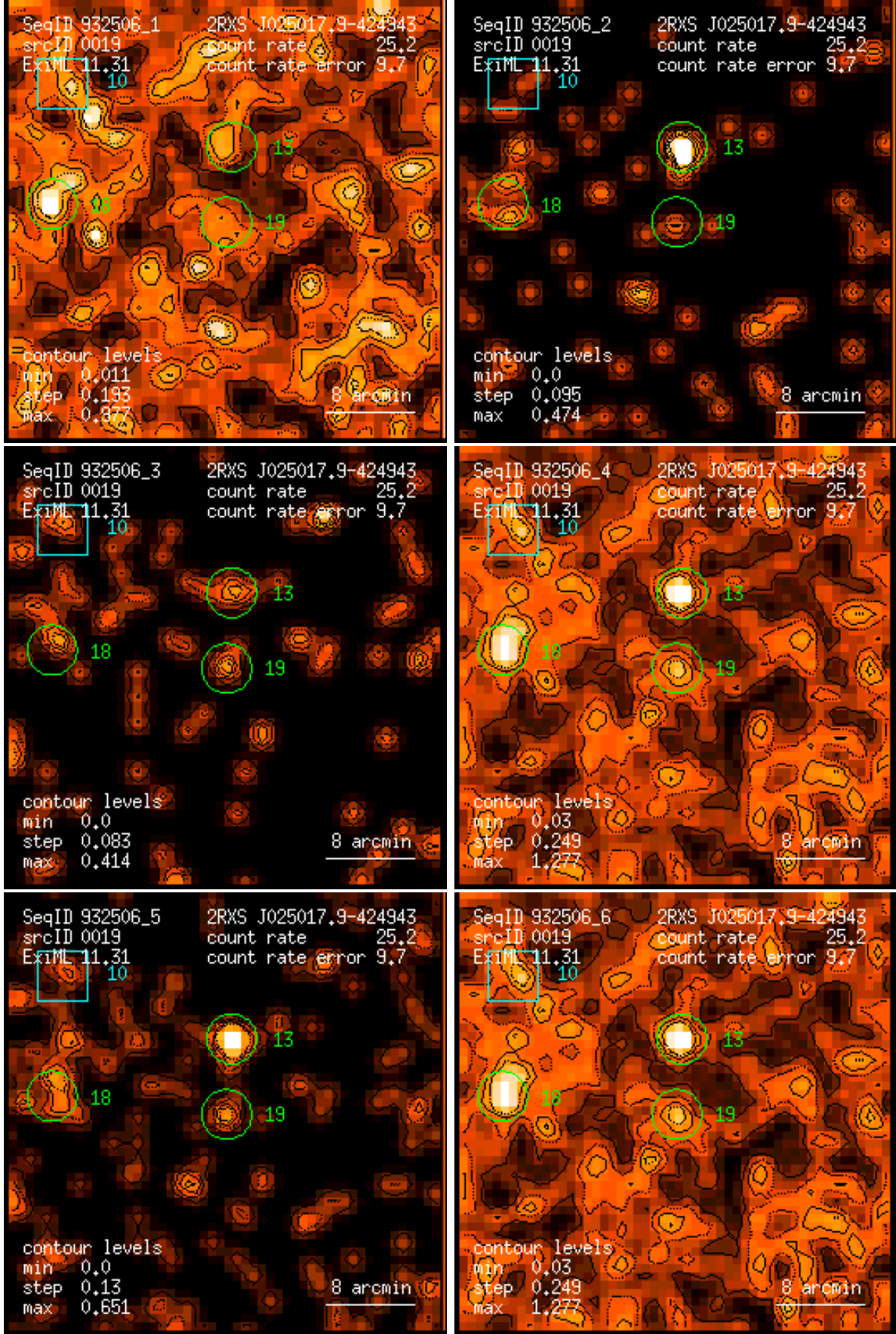
Figure 19: RASS 932506: detection 0019: band rate images, Gaussian filter: (1) PSPC channels 11 – 41, (2) 52 – 90, (3) 91 – 201, (4) 11 – 235, (5) 52 – 201, (6) 11 – 201. Broad band rates in counts/ks. Band rate contour levels in counts/ks/arcmin 2 .
