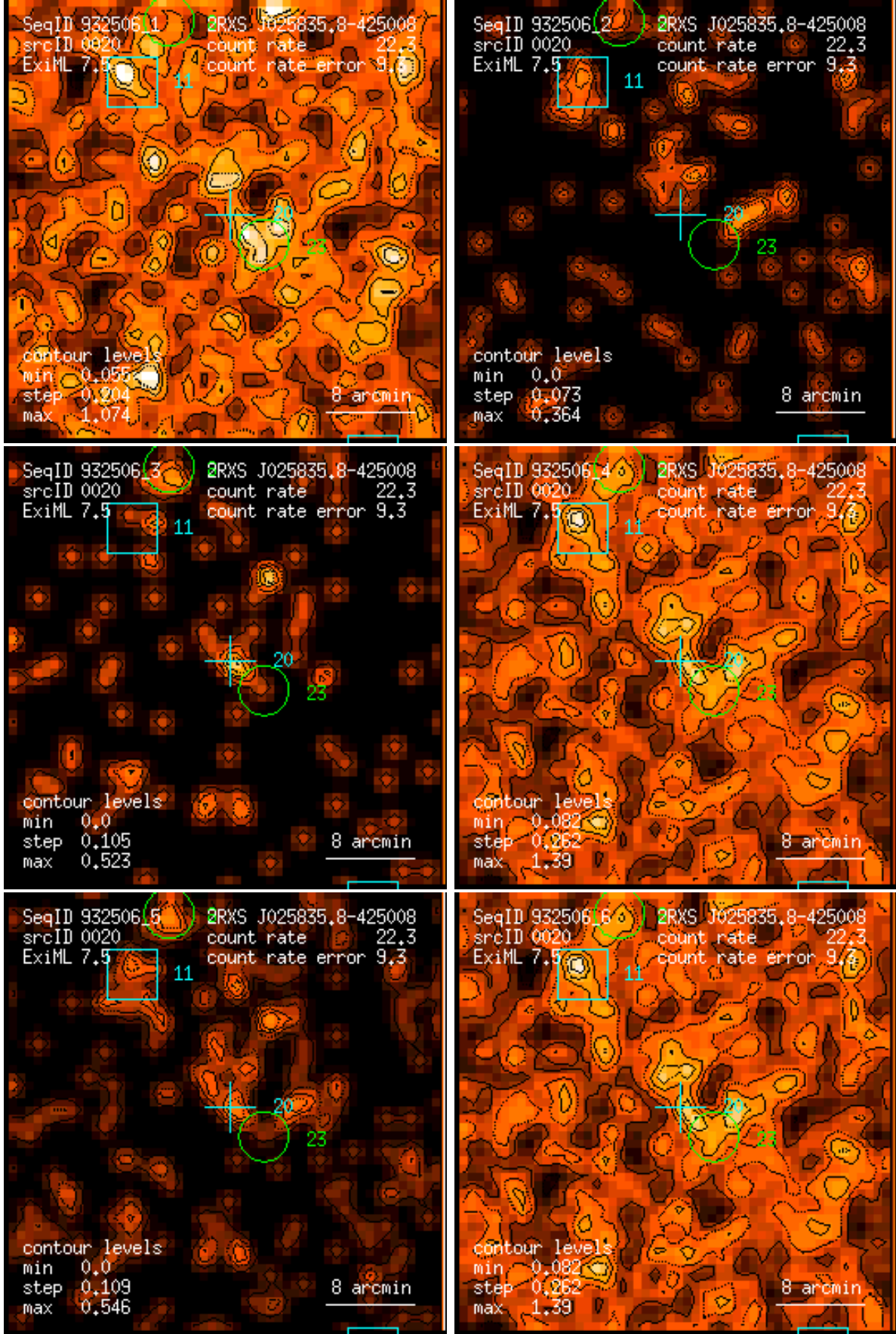
Figure 20: RASS 932506: detection 0020: band rate images, Gaussian filter: (1) PSPC channels 11 – 41, (2) 52 – 90, (3) 91 – 201, (4) 11 – 235, (5) 52 – 201, (6) 11 – 201. Broad band rates in counts/ks. Band rate contour levels in counts/ks/arcmin 2 .
