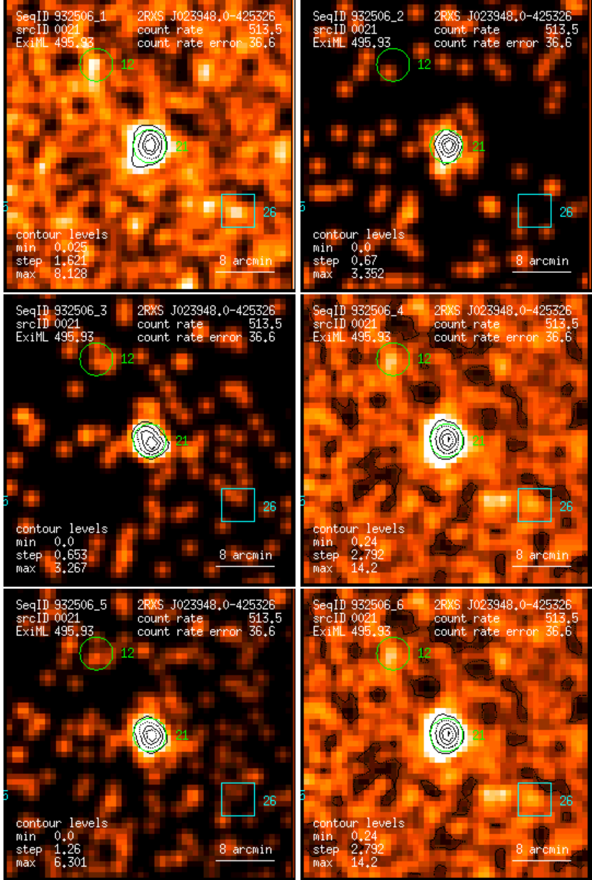
Figure 21: RASS 932506: detection 0021: band rate images, Gaussian filter: (1) PSPC channels 11 – 41, (2) 52 – 90, (3) 91 – 201, (4) 11 – 235, (5) 52 – 201, (6) 11 – 201. Broad band rates in counts/ks. Band rate contour levels in counts/ks/arcmin 2 .
