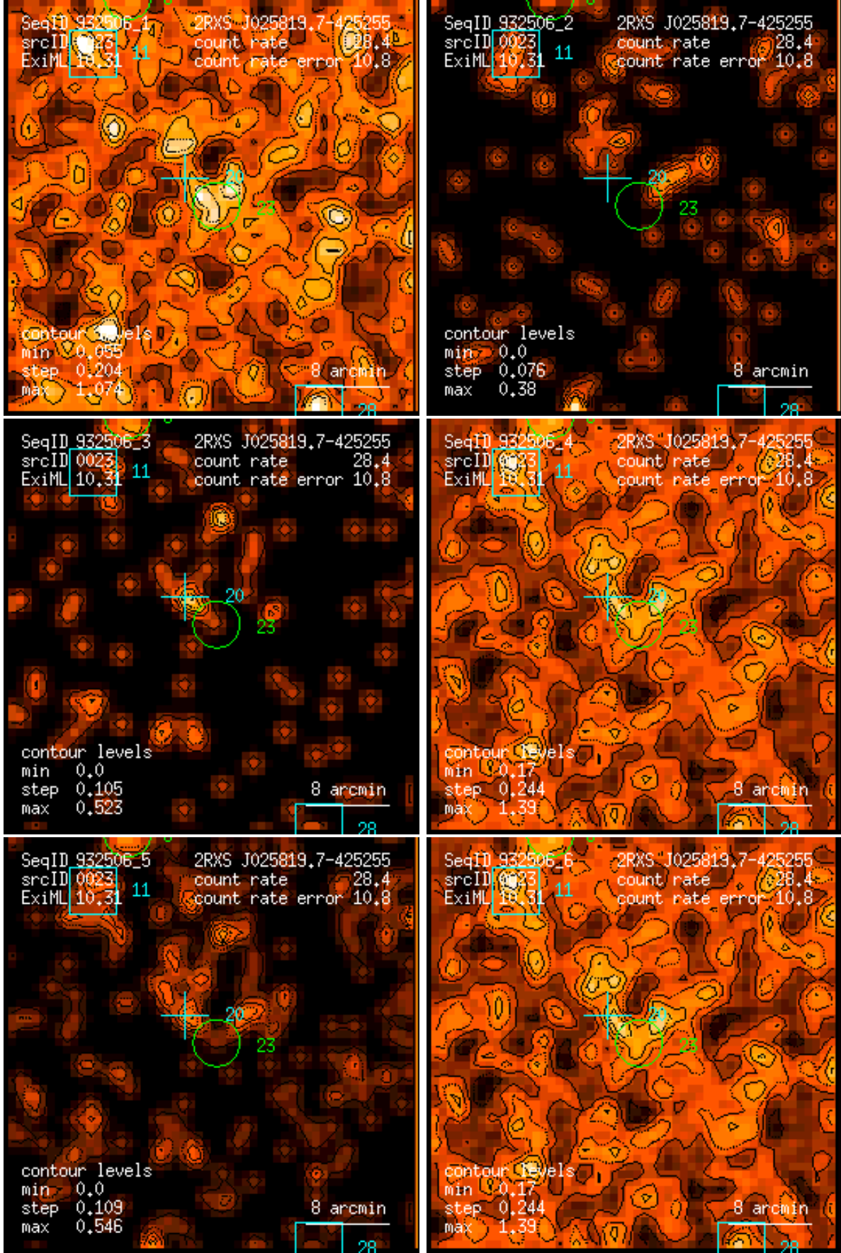
Figure 23: RASS 932506: detection 0023: band rate images, Gaussian filter: (1) PSPC channels 11 – 41, (2) 52 – 90, (3) 91 – 201, (4) 11 – 235, (5) 52 – 201, (6) 11 – 201. Broad band rates in counts/ks. Band rate contour levels in counts/ks/arcmin 2 .
