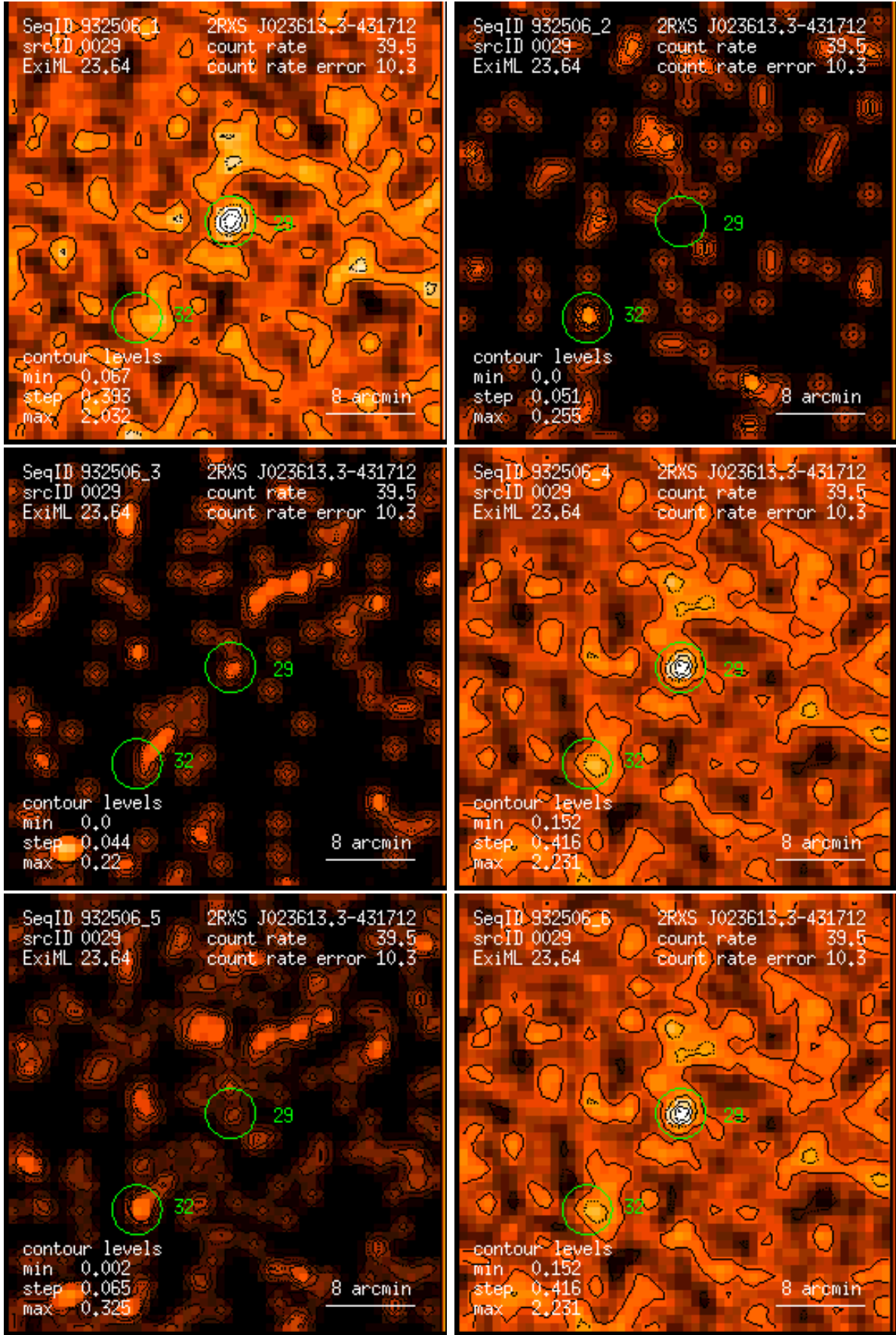
Figure 29: RASS 932506: detection 0029: band rate images, Gaussian filter: (1) PSPC channels 11 – 41, (2) 52 – 90, (3) 91 – 201, (4) 11 – 235, (5) 52 – 201, (6) 11 – 201. Broad band rates in counts/ks. Band rate contour levels in counts/ks/arcmin 2 .
