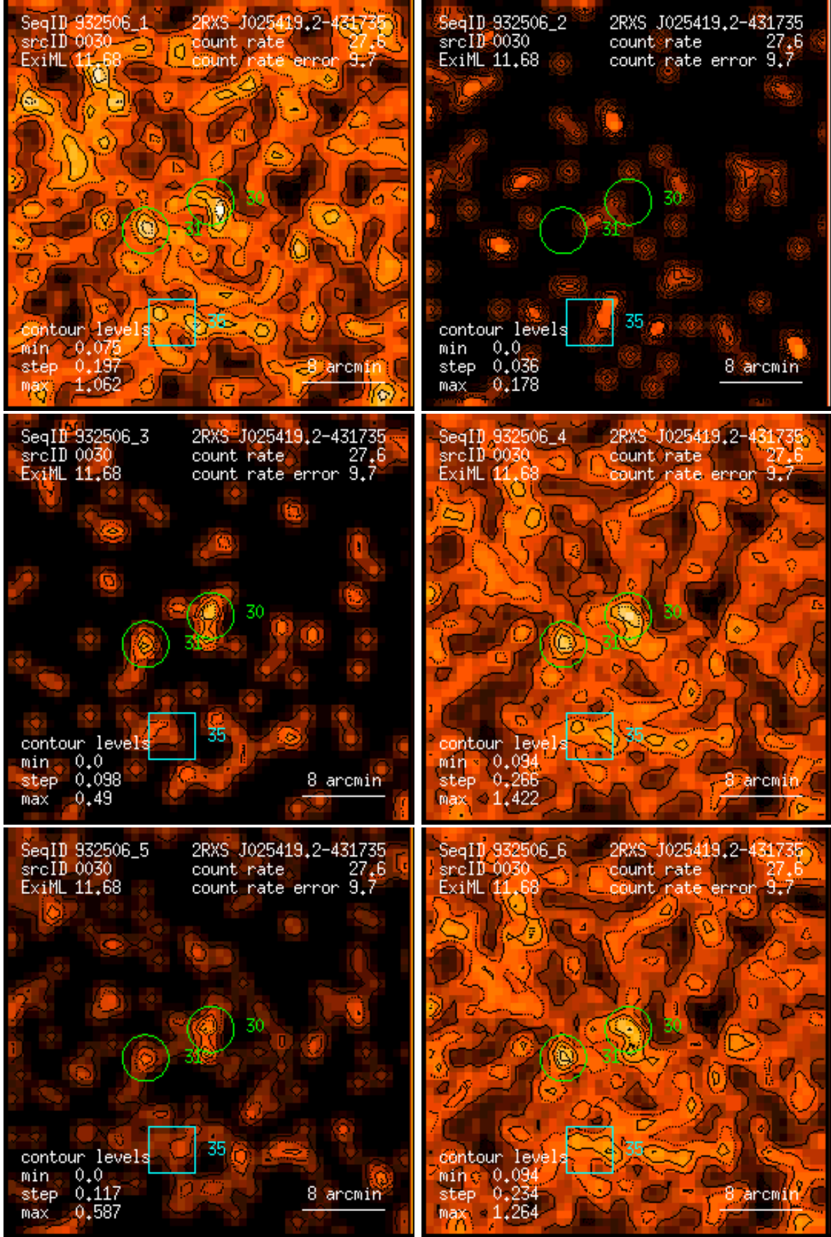
Figure 30: RASS 932506: detection 0030: band rate images, Gaussian filter: (1) PSPC channels 11 – 41, (2) 52 – 90, (3) 91 – 201, (4) 11 – 235, (5) 52 – 201, (6) 11 – 201. Broad band rates in counts/ks. Band rate contour levels in counts/ks/arcmin 2 .
