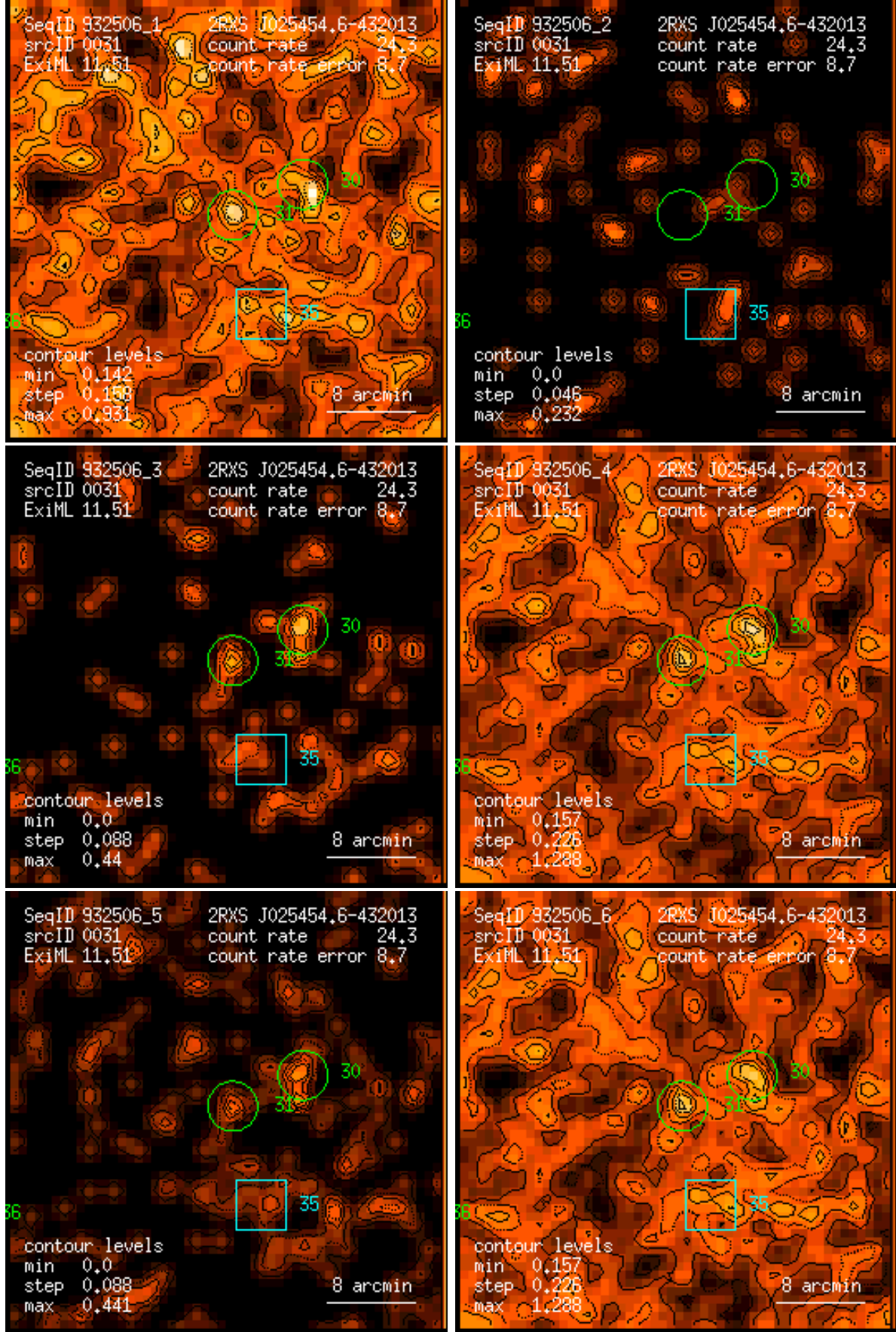
Figure 31: RASS 932506: detection 0031: band rate images, Gaussian filter: (1) PSPC channels 11 – 41, (2) 52 – 90, (3) 91 – 201, (4) 11 – 235, (5) 52 – 201, (6) 11 – 201. Broad band rates in counts/ks. Band rate contour levels in counts/ks/arcmin 2 .
