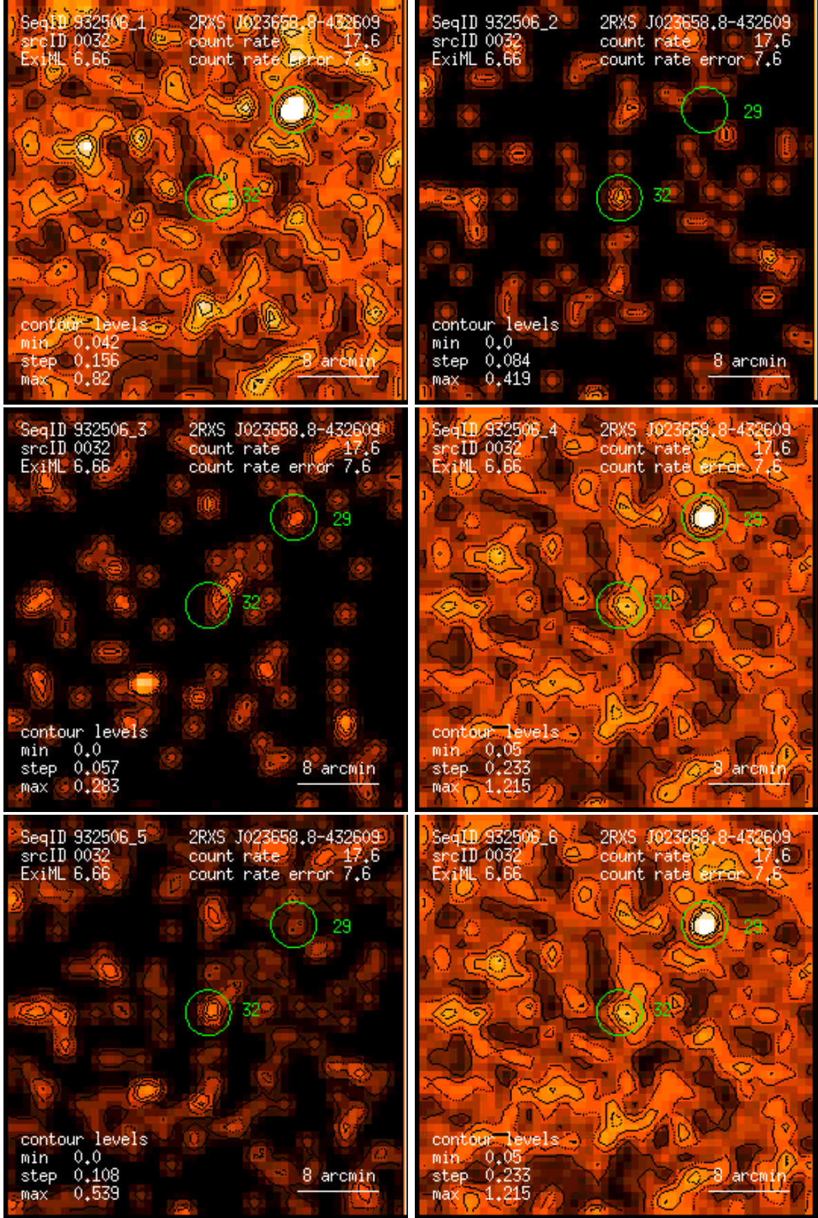
Figure 32: RASS 932506: detection 0032: band rate images, Gaussian filter: (1) PSPC channels 11 – 41, (2) 52 – 90, (3) 91 – 201, (4) 11 – 235, (5) 52 – 201, (6) 11 – 201. Broad band rates in counts/ks. Band rate contour levels in counts/ks/arcmin 2 .
