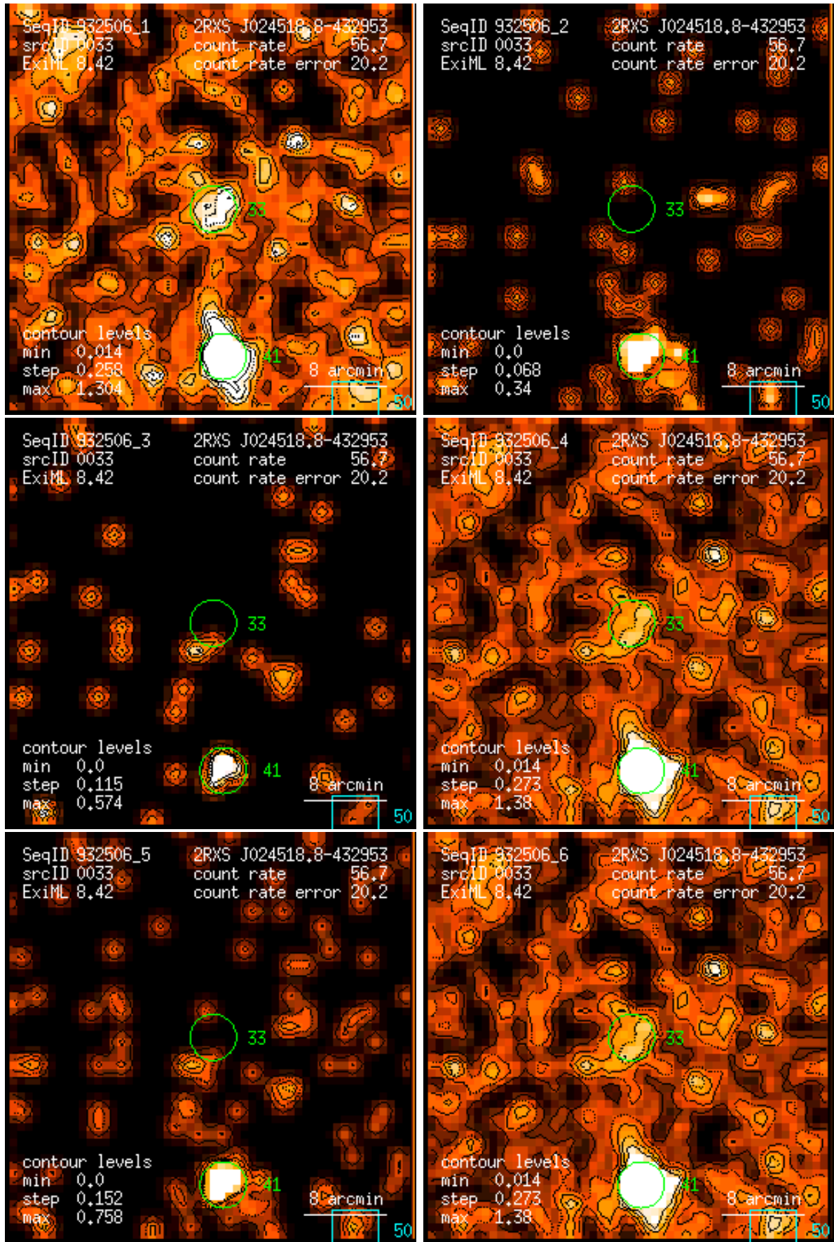
Figure 33: RASS 932506: detection 0033: band rate images, Gaussian filter: (1) PSPC channels 11 – 41, (2) 52 – 90, (3) 91 – 201, (4) 11 – 235, (5) 52 – 201, (6) 11 – 201. Broad band rates in counts/ks. Band rate contour levels in counts/ks/arcmin 2 .
