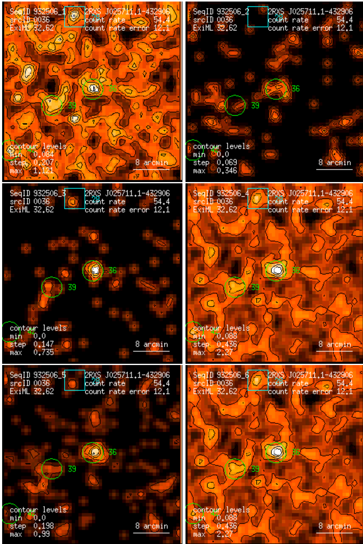
Figure 36: RASS 932506: detection 0036: band rate images, Gaussian filter: (1) PSPC channels 11 – 41, (2) 52 – 90, (3) 91 – 201, (4) 11 – 235, (5) 52 – 201, (6) 11 – 201. Broad band rates in counts/ks. Band rate contour levels in counts/ks/arcmin 2 .
