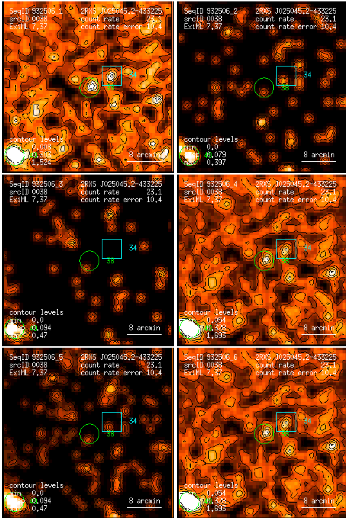
Figure 38: RASS 932506: detection 0038: band rate images, Gaussian filter: (1) PSPC channels 11 – 41, (2) 52 – 90, (3) 91 – 201, (4) 11 – 235, (5) 52 – 201, (6) 11 – 201. Broad band rates in counts/ks. Band rate contour levels in counts/ks/arcmin 2 .
