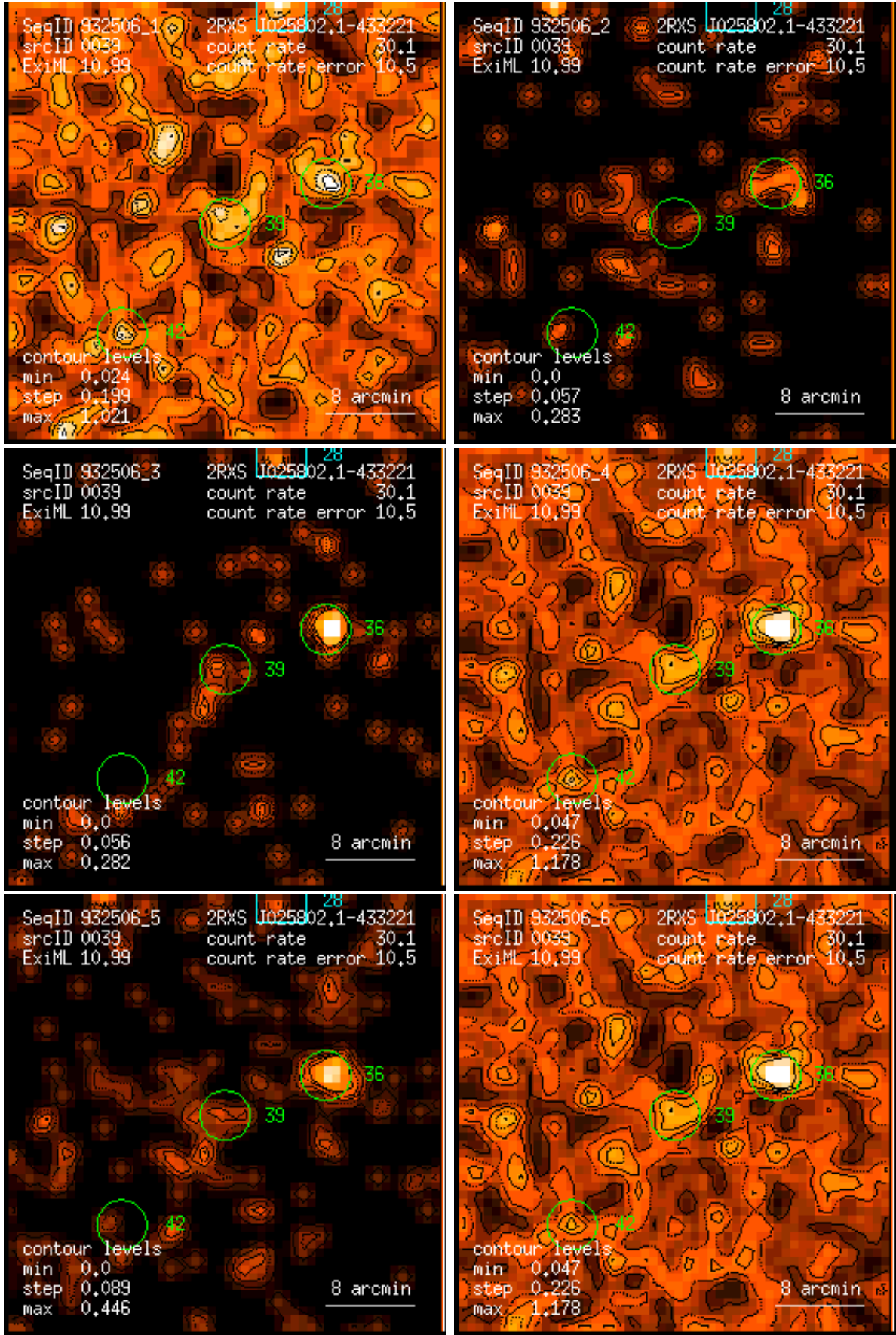
Figure 39: RASS 932506: detection 0039: band rate images, Gaussian filter: (1) PSPC channels 11 – 41, (2) 52 – 90, (3) 91 – 201, (4) 11 – 235, (5) 52 – 201, (6) 11 – 201. Broad band rates in counts/ks. Band rate contour levels in counts/ks/arcmin 2 .
