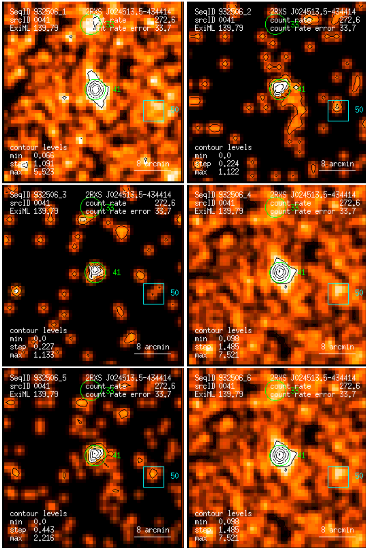
Figure 41: RASS 932506: detection 0041: band rate images, Gaussian filter: (1) PSPC channels 11 – 41, (2) 52 – 90, (3) 91 – 201, (4) 11 – 235, (5) 52 – 201, (6) 11 – 201. Broad band rates in counts/ks. Band rate contour levels in counts/ks/arcmin 2 .
