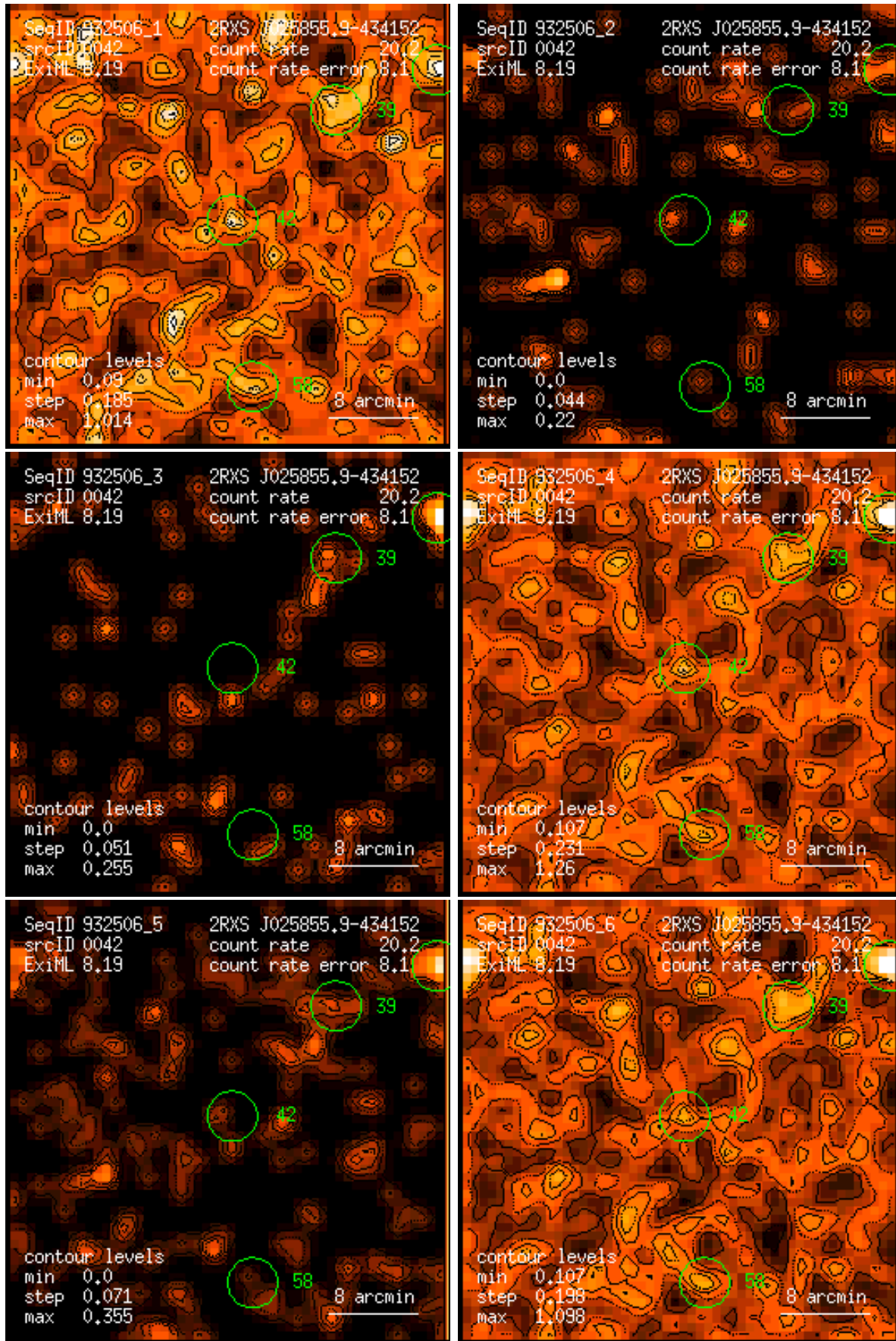
Figure 42: RASS 932506: detection 0042: band rate images, Gaussian filter: (1) PSPC channels 11 – 41, (2) 52 – 90, (3) 91 – 201, (4) 11 – 235, (5) 52 – 201, (6) 11 – 201. Broad band rates in counts/ks. Band rate contour levels in counts/ks/arcmin 2 .
