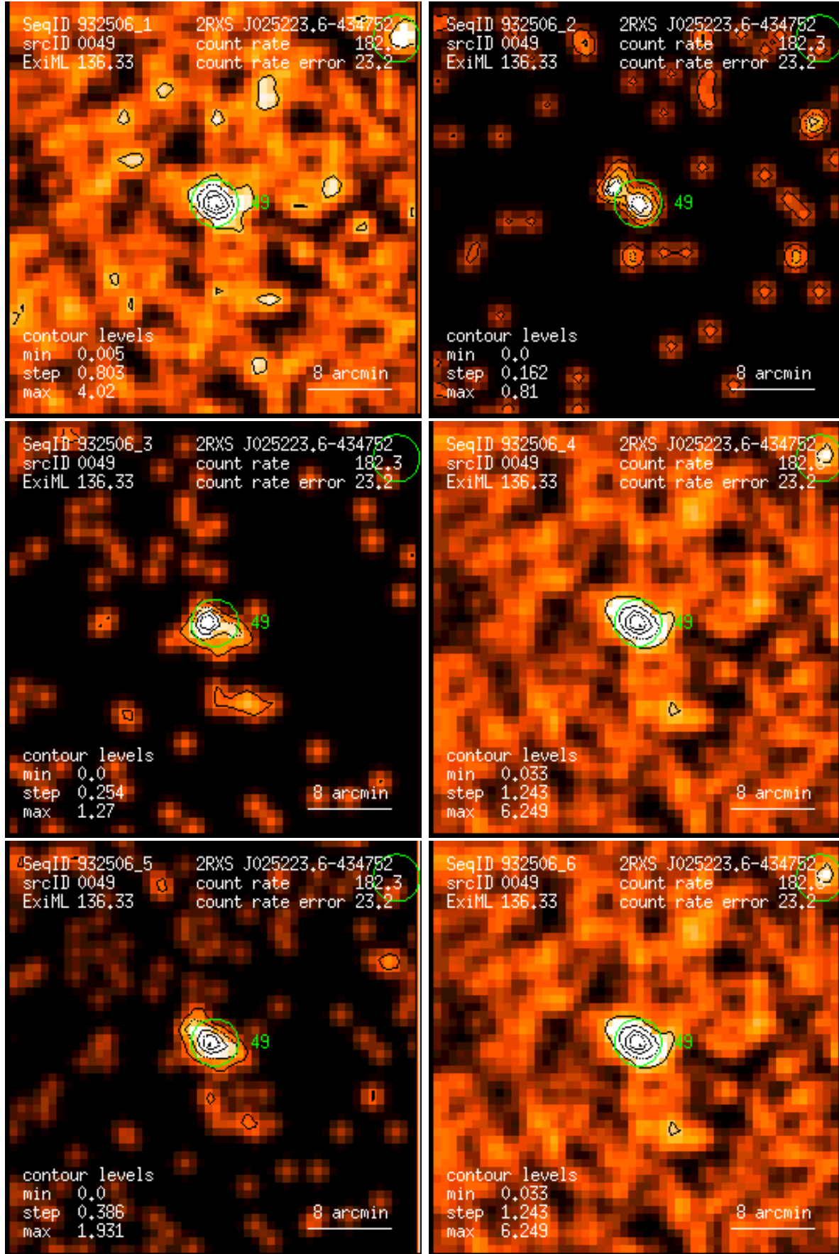
Figure 49: RASS 932506: detection 0049: band rate images, Gaussian filter: (1) PSPC channels 11 – 41, (2) 52 – 90, (3) 91 – 201, (4) 11 – 235, (5) 52 – 201, (6) 11 – 201. Broad band rates in counts/ks. Band rate contour levels in counts/ks/arcmin 2 .
