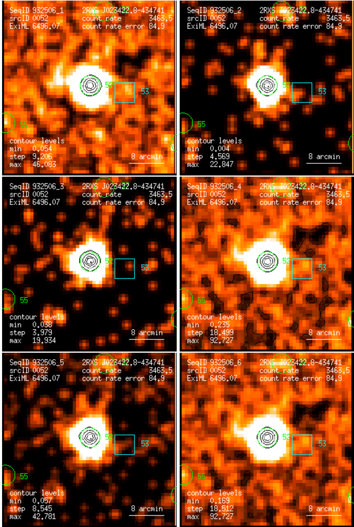
Figure 52: RASS 932506: detection 0052: band rate images, Gaussian filter: (1) PSPC channels 11 – 41, (2) 52 – 90, (3) 91 – 201, (4) 11 – 235, (5) 52 – 201, (6) 11 – 201. Broad band rates in counts/ks. Band rate contour levels in counts/ks/arcmin 2 .
