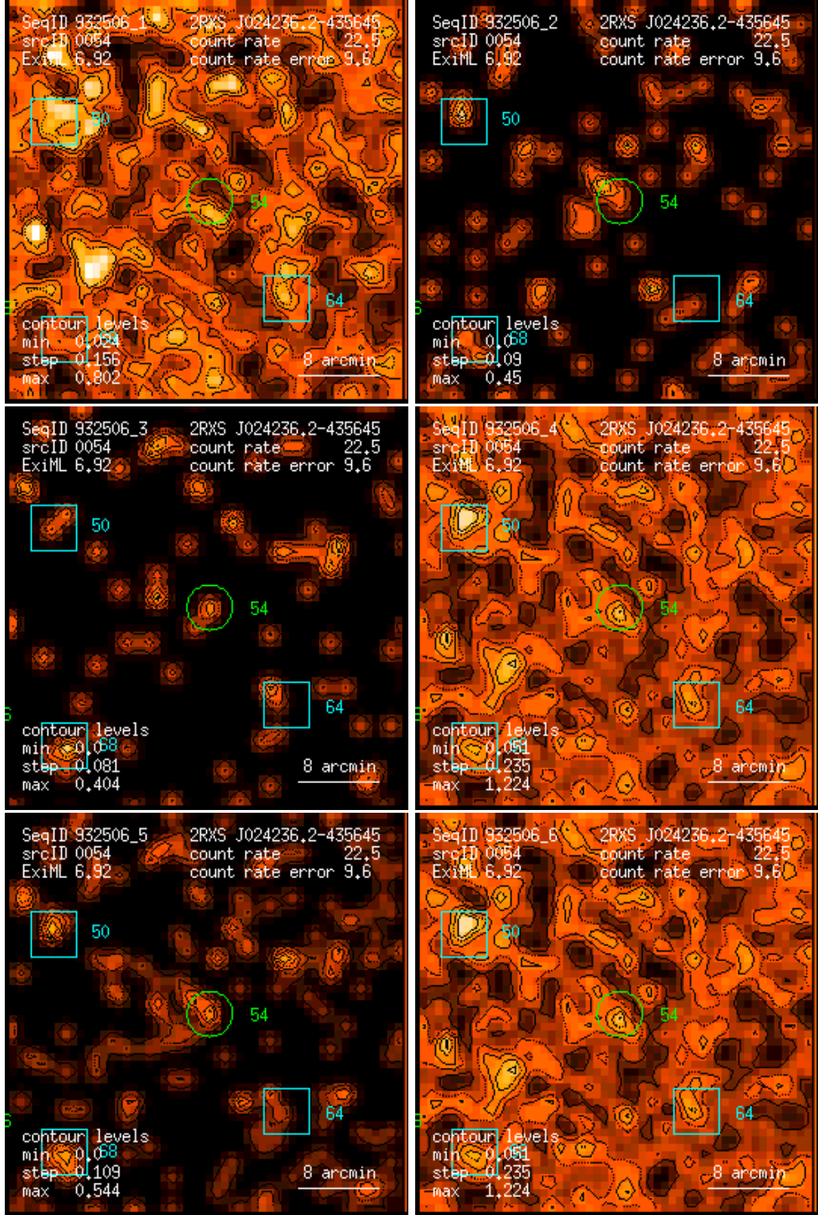
Figure 54: RASS 932506: detection 0054: band rate images, Gaussian filter: (1) PSPC channels 11 – 41, (2) 52 – 90, (3) 91 – 201, (4) 11 – 235, (5) 52 – 201, (6) 11 – 201. Broad band rates in counts/ks. Band rate contour levels in counts/ks/arcmin 2 .
