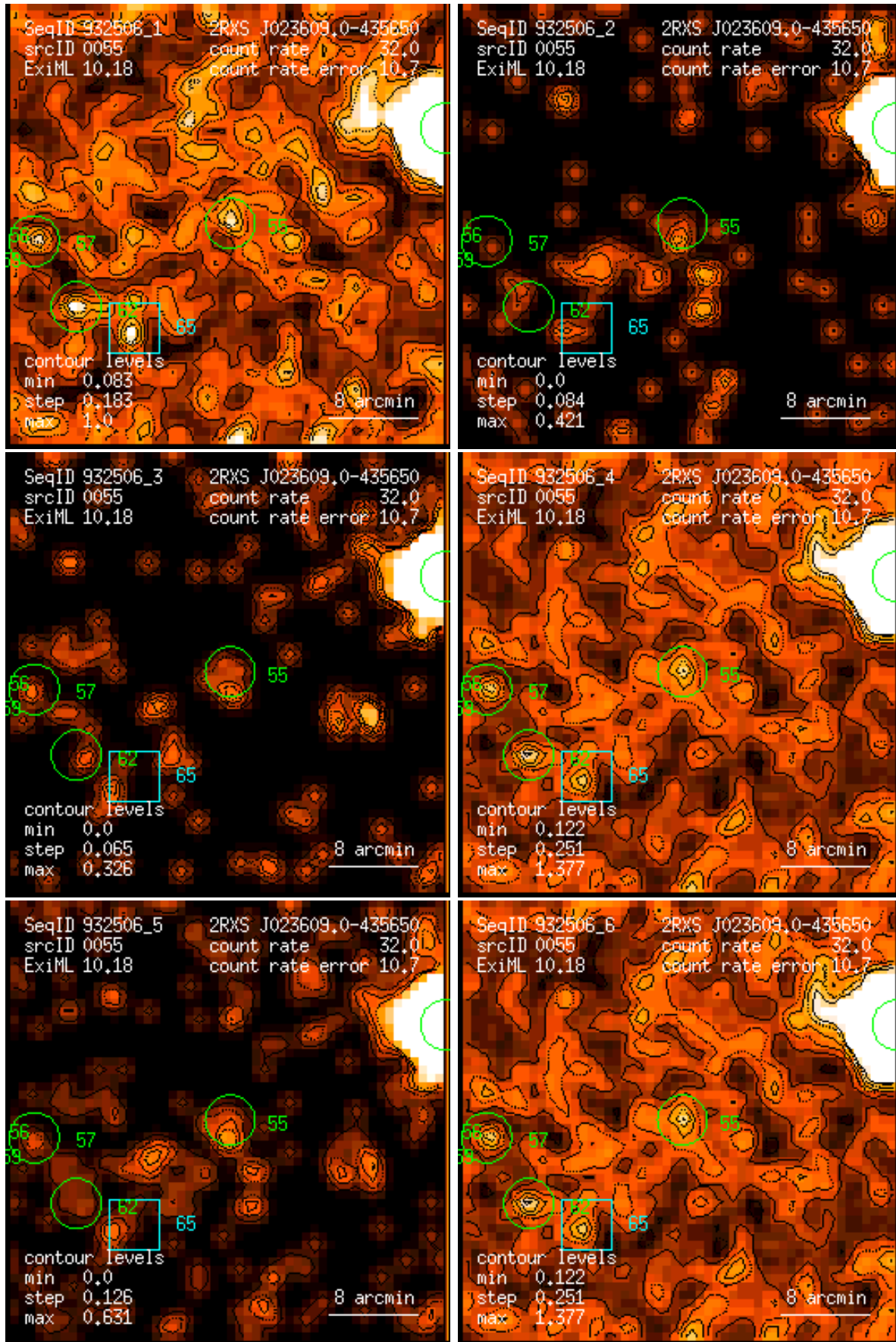
Figure 55: RASS 932506: detection 0055: band rate images, Gaussian filter: (1) PSPC channels 11 – 41, (2) 52 – 90, (3) 91 – 201, (4) 11 – 235, (5) 52 – 201, (6) 11 – 201. Broad band rates in counts/ks. Band rate contour levels in counts/ks/arcmin 2 .
