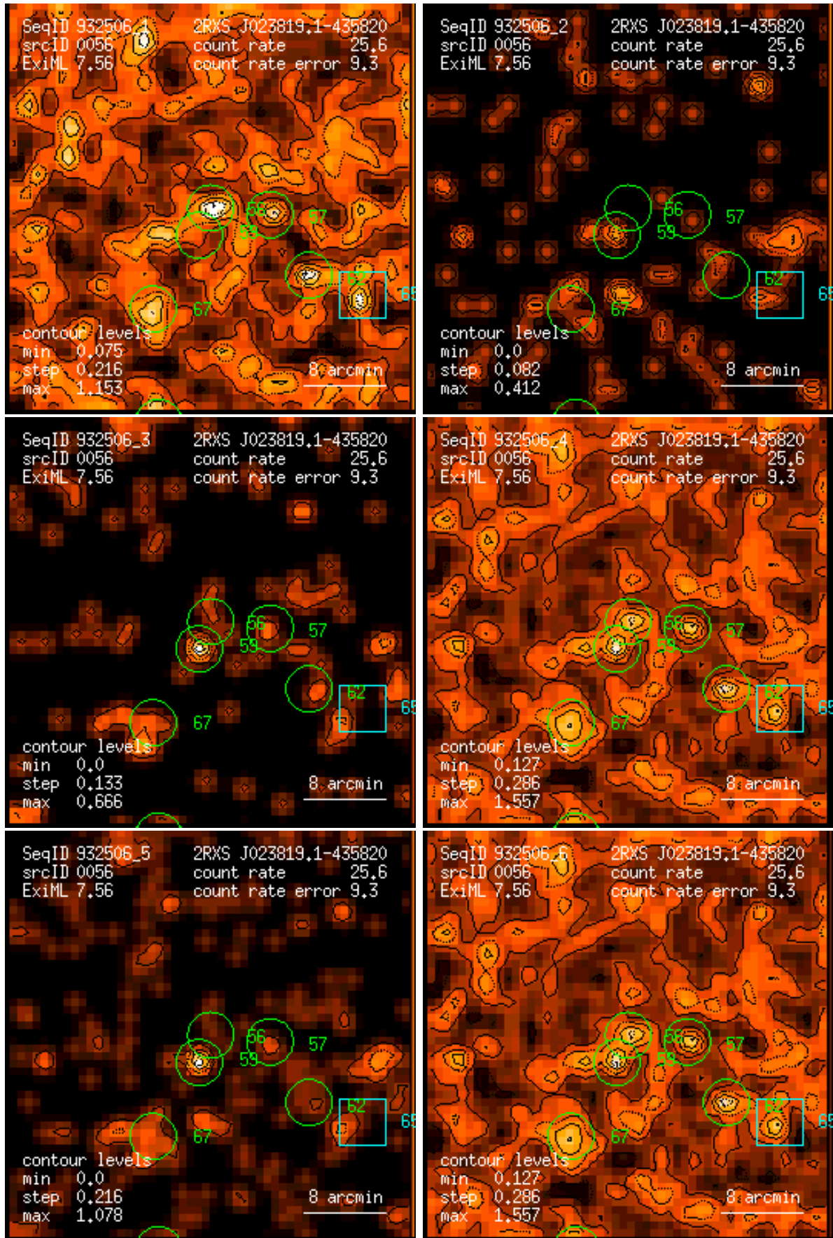
Figure 56: RASS 932506: detection 0056: band rate images, Gaussian filter: (1) PSPC channels 11 – 41, (2) 52 – 90, (3) 91 – 201, (4) 11 – 235, (5) 52 – 201, (6) 11 – 201. Broad band rates in counts/ks. Band rate contour levels in counts/ks/arcmin 2 .
