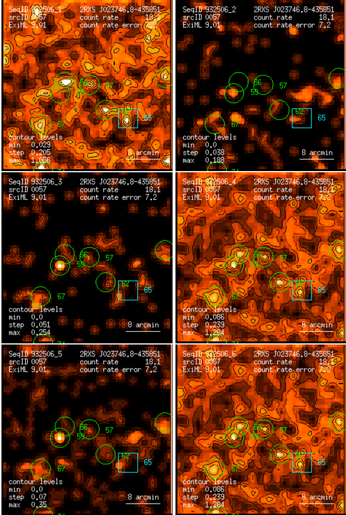
Figure 57: RASS 932506: detection 0057: band rate images, Gaussian filter: (1) PSPC channels 11 – 41, (2) 52 – 90, (3) 91 – 201, (4) 11 – 235, (5) 52 – 201, (6) 11 – 201. Broad band rates in counts/ks. Band rate contour levels in counts/ks/arcmin 2 .
