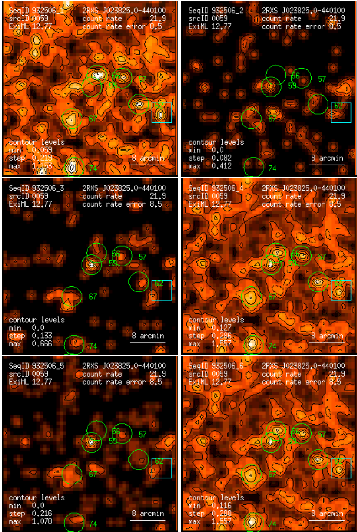
Figure 59: RASS 932506: detection 0059: band rate images, Gaussian filter: (1) PSPC channels 11 – 41, (2) 52 – 90, (3) 91 – 201, (4) 11 – 235, (5) 52 – 201, (6) 11 – 201. Broad band rates in counts/ks. Band rate contour levels in counts/ks/arcmin 2 .
