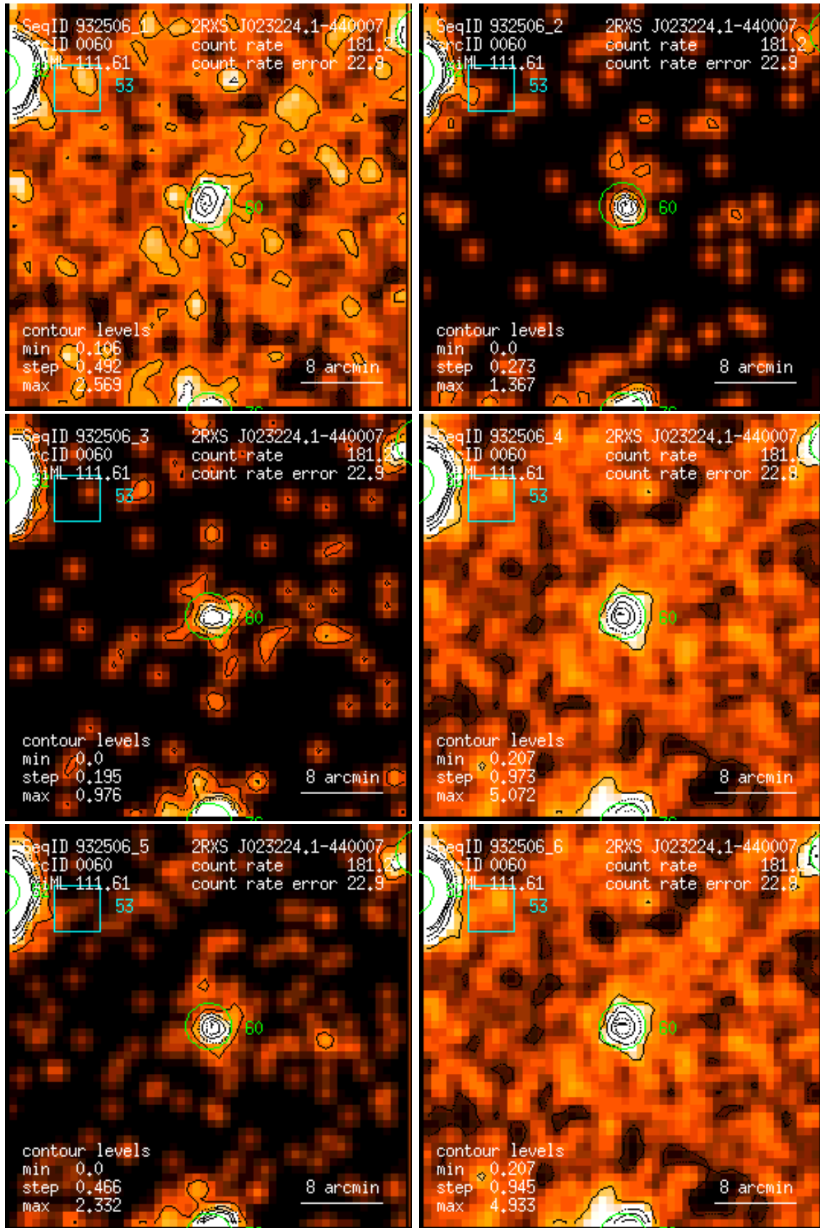
Figure 60: RASS 932506: detection 0060: band rate images, Gaussian filter: (1) PSPC channels 11 – 41, (2) 52 – 90, (3) 91 – 201, (4) 11 – 235, (5) 52 – 201, (6) 11 – 201. Broad band rates in counts/ks. Band rate contour levels in counts/ks/arcmin 2 .
