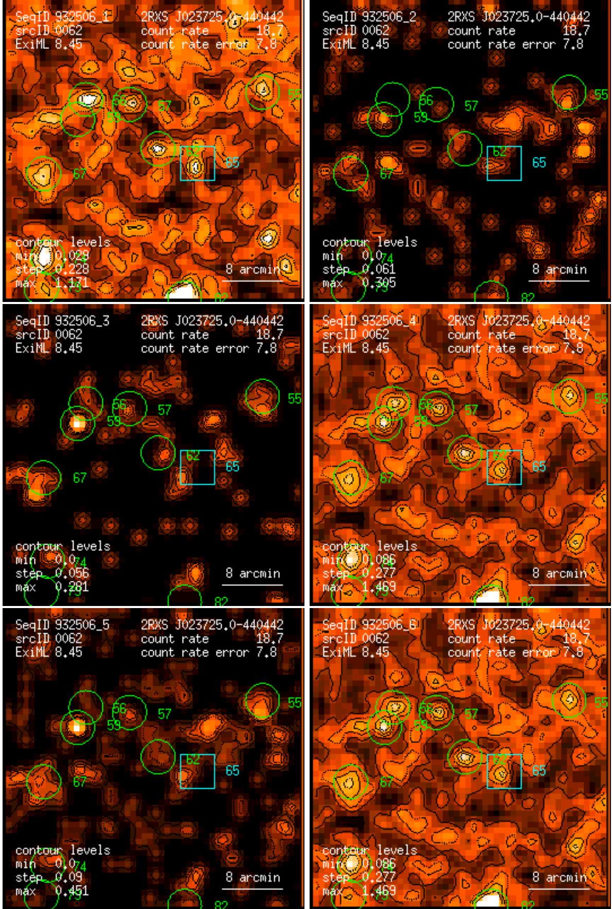
Figure 62: RASS 932506: detection 0062: band rate images, Gaussian filter: (1) PSPC channels 11 – 41, (2) 52 – 90, (3) 91 – 201, (4) 11 – 235, (5) 52 – 201, (6) 11 – 201. Broad band rates in counts/ks. Band rate contour levels in counts/ks/arcmin 2 .
