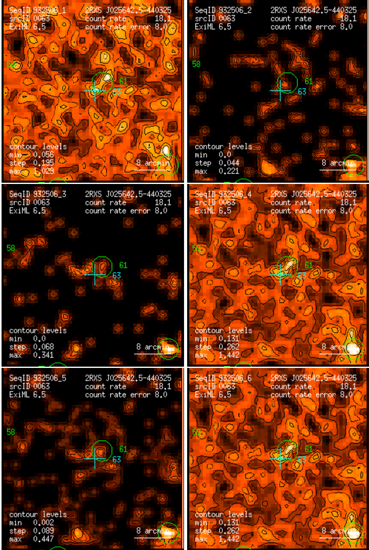
Figure 63: RASS 932506: detection 0063: band rate images, Gaussian filter: (1) PSPC channels 11 – 41, (2) 52 – 90, (3) 91 – 201, (4) 11 – 235, (5) 52 – 201, (6) 11 – 201. Broad band rates in counts/ks. Band rate contour levels in counts/ks/arcmin 2 .
