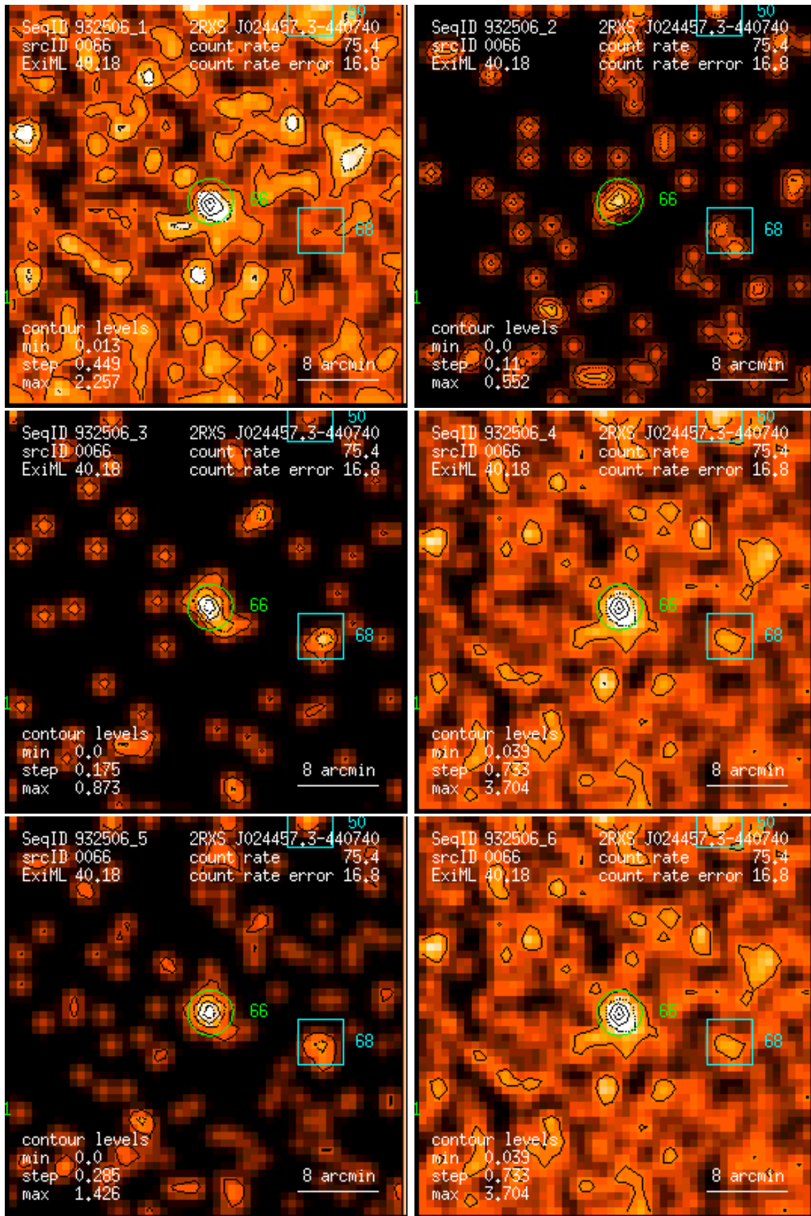
Figure 66: RASS 932506: detection 0066: band rate images, Gaussian filter: (1) PSPC channels 11 – 41, (2) 52 – 90, (3) 91 – 201, (4) 11 – 235, (5) 52 – 201, (6) 11 – 201. Broad band rates in counts/ks. Band rate contour levels in counts/ks/arcmin 2 .
