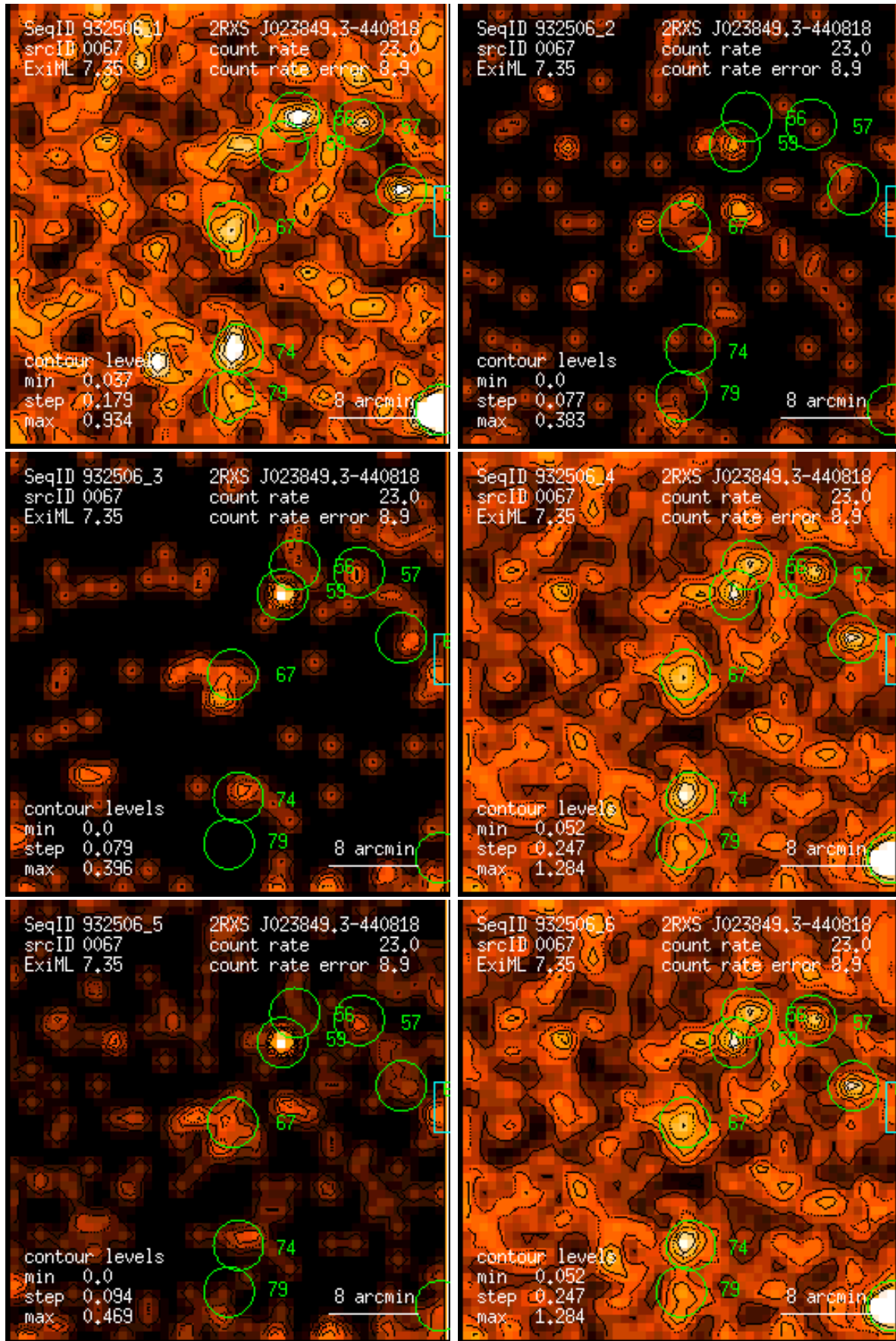
Figure 67: RASS 932506: detection 0067: band rate images, Gaussian filter: (1) PSPC channels 11 – 41, (2) 52 – 90, (3) 91 – 201, (4) 11 – 235, (5) 52 – 201, (6) 11 – 201. Broad band rates in counts/ks. Band rate contour levels in counts/ks/arcmin 2 .
